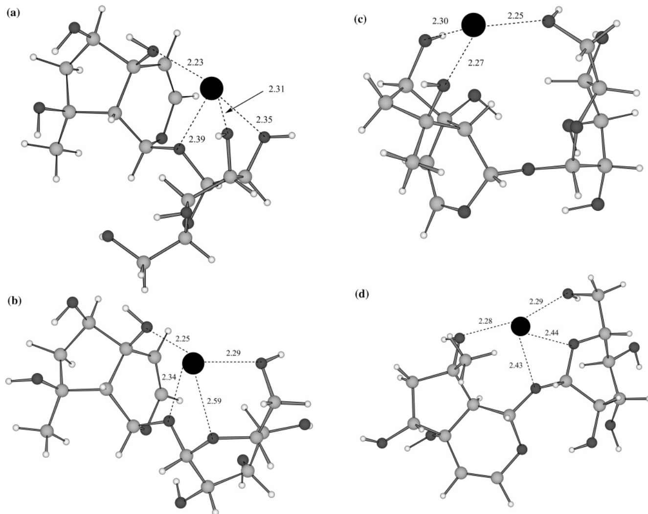
Figure 4. (a) Geometry of HarNa + I optimized at the B3LYP/6-31G* level; distances are in Å. (b) Geometry of HarNa + II optimized at the B3LYP/6-31G* level; distances are in Å. (c) Geometry of HarNa + III optimized at the B3LYP/6-31G* level; distances are in Å. (d) Geometry of HarNa + IV optimized at the B3LYP/6-31G* level; distances are in Å.
