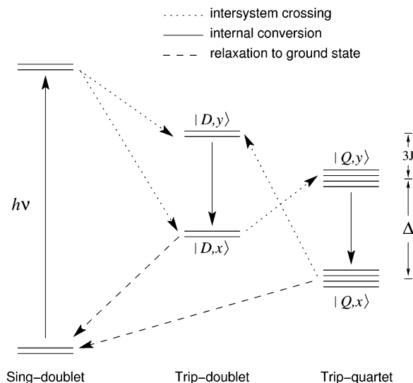
Figure 1. A simplified Jablonski diagram of OEPVO showing the low-lying states of the sing-doublet, trip-doublet, and trip-quartet manifolds. The relative energies of the states is not to scale, and the energy differences between the trip-doublet and trip-quartet states has been greatly expanded. The labels x and y refer to states derived from excitation of an electron from the HOMO into the e_x and e_y orbitals, respectively.
