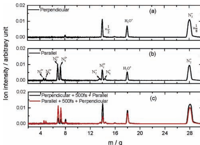
Figure 3. TOF mass spectra of N 2 irradiated by 800-nm, 110-fs laser pulses (a) perpendicular polarized laser alone; (b) parallel polarized laser alone; (c) double pulse with perpendicular polarized laser preceding parallel polarized laser by 500 fs (black line) and double pulse with parallel polarized laser preceding perpendicular polarized laser by 500 fs (red line). The laser intensities were 6 \times 10^{14} W/cm 2 for both perpendicular and parallel laser pulses.
