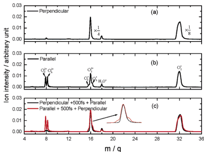
Figure 2. TOF mass spectra of O 2 irradiated by 800-nm, 110-fs laser pulses (a) perpendicular polarized laser alone; (b) parallel polarized laser alone; (c) double pulse with perpendicular polarized laser preceding parallel polarized laser by 500 fs (black line) and double pulse with parallel polarized laser preceding perpendicular polarized laser by 500 fs (red line). The laser intensities were 6 \times 10^{14} W/cm 2 for both perpendicular and parallel laser pulses.
