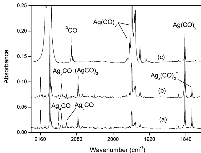
Figure 2. IR spectra in the 2160–1800 cm -1 region for laser-ablated Ag atoms co-deposited with different CO concentration and laser power after annealing to 30 K in Ar: (a) 0.02% CO and 12 mJ/pulse, (b) 0.03% CO and 10 mJ/pulse, and (c) 0.4% CO and 7 mJ/pulse.
