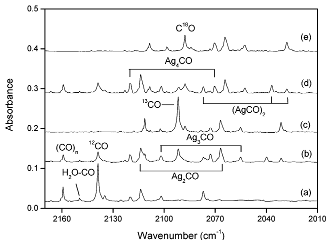
Figure 3. IR spectra in the 2160–2010 \text{cm}^{-1} region for laser-ablated (12 mJ/pulse) Ag atoms co-deposited with isotopic CO in Ar after annealing to 30 K: (a) 0.02% ^{12}\text{C}^{16}\text{O} , (b) 0.01% ^{12}\text{C}^{16}\text{O} + 0.01% ^{13}\text{C}^{16}\text{O} , (c) 0.02% ^{13}\text{C}^{16}\text{O} , (d) 0.01% ^{12}\text{C}^{16}\text{O} + 0.01% ^{12}\text{C}^{18}\text{O} , and (e) 0.02% ^{12}\text{C}^{18}\text{O} .
