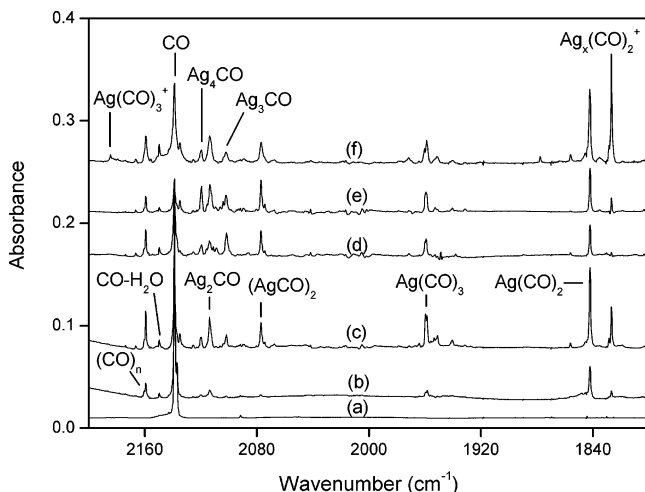
Figure 1. IR spectra in the 2160–1800 cm -1 region from co-deposition of laser-ablated (12 mJ/pulse) Ag atoms with 0.02% CO in Ar: (a) 1 h of sample deposition at 7 K, (b) after annealing to 25 K, (c) after annealing to 30 K, (d) after 15 min of broad-band irradiation, (e) after annealing to 35 K, and (f) 0.02% CO + 0.005% CCl 4 , after annealing to 30 K.
