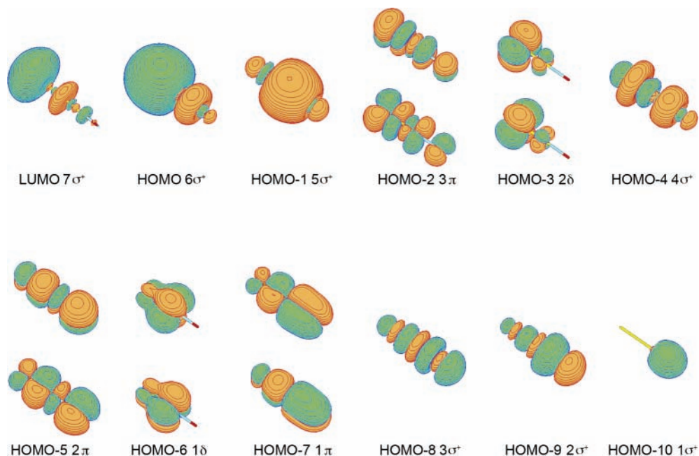
Figure 7. Molecular orbitals of Au_2BO^- C_{\infty v} (^1\Sigma^+) .
