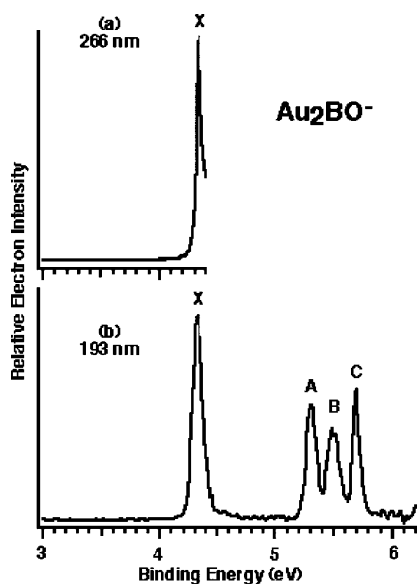
Figure 2. Photoelectron spectra of \text{Au}_2\text{BO}^- at (a) 266 and (b) 193 nm.
