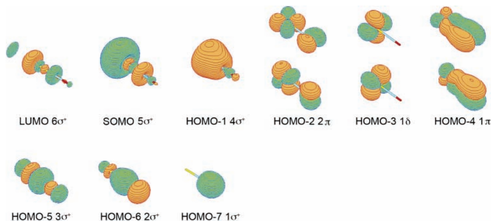
Figure 5. Molecular orbitals of AuBO - C ∞v ( 2 Σ + ).
