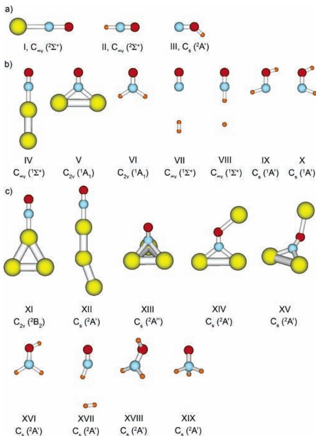
Figure 4. Structures of the most stable isomers of auro-borane oxides \text{Au}_n\text{BO}^- ( n = 1-3 ) and boron hydride oxides \text{H}_n\text{BO}^- ( n = 1-3 ): (a) \text{AuBO}^- and \text{HBO}^- , (b) \text{Au}_2\text{BO}^- and \text{H}_2\text{BO}^- , and (c) \text{Au}_3\text{BO}^- and \text{H}_3\text{BO}^- .
