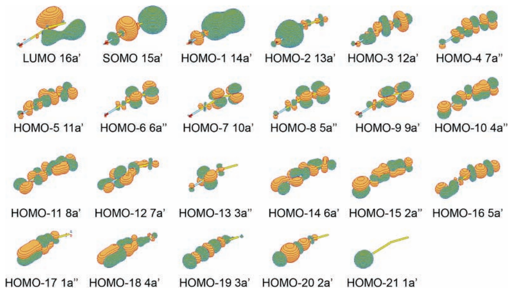
Figure 9. Molecular orbitals of \text{Au}_3\text{BO}^- C_s ({}^2A') .
