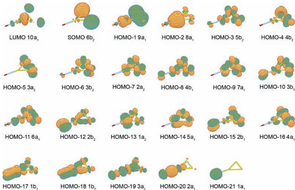
Figure 8. Molecular orbitals of Au_3BO^- C_{2v} (^2B_2) .
