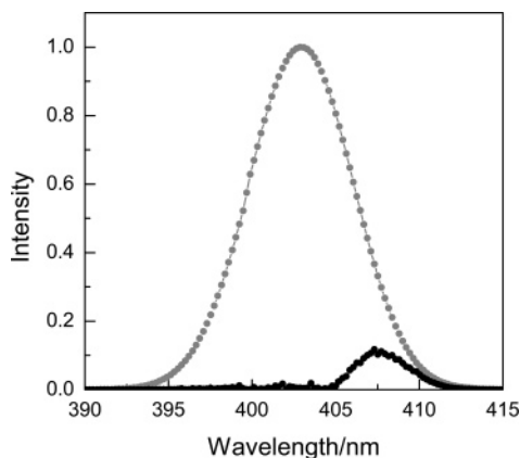
Figure 5. Calculated SH spectrum of the best pulse from generation 299 of the simulation (black). This is shown relative to the calculated normalized SH spectrum of a bandwidth-limited pulse (gray).
