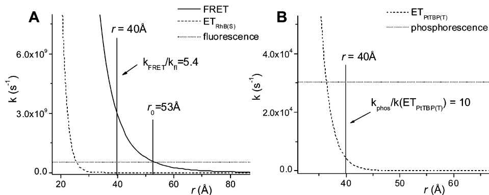
Figure 4. Calculated distance dependences of FRET, ET_{RhB(S)} (A) and ET_{PtTBP(T)} (B), in RhB–PtTBP systems.
