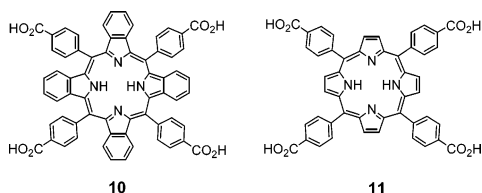
Figure 8. Fluorescent free-base porphyrins used to evaluate 2PA cross sections of Pt tetraaryltetrabenzoporphyrins 1 and 2 .
