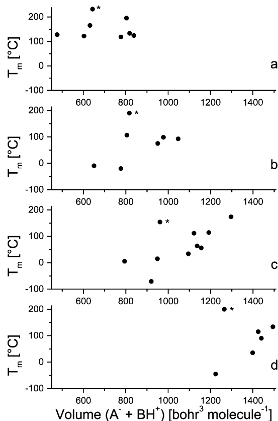
Figure 4. T_m versus volume ( A^- + BH^+ ) for (a) ammonia based PILs, (b) MA based PILs, (c) EA based PILs, and (d) BA based PILs, respectively. The PIL with BF_4^- as the anion (marked with *) has a T_m higher than the trend-line for all cations.
