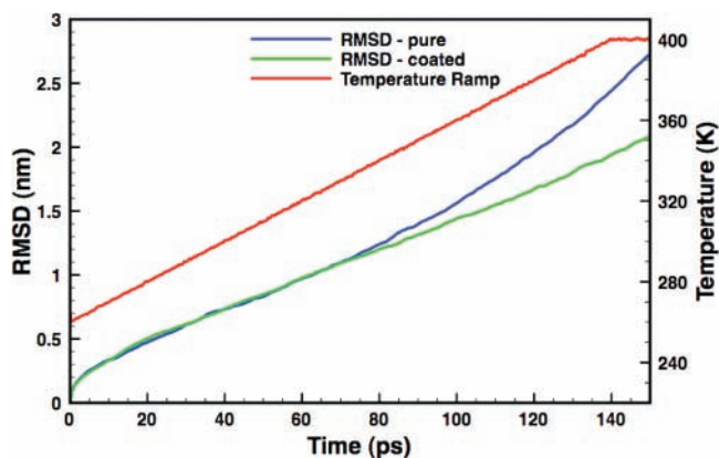
Figure 4. Root-mean-square deviations of water molecules in the pure and coated particles during a heating ramp (red line).
