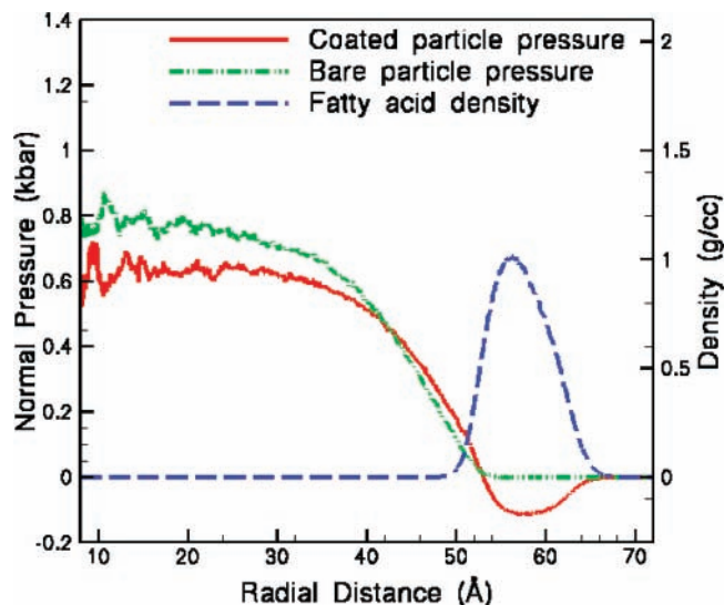
Figure 1. Pressure profiles of bare and coated particles. The dashed (blue) curve represents the fatty acid density. It is evident from the plot that while the interior of the particle is under compression, the coating is under negative pressure, i.e., tension. Reprinted from ref 8. Copyright 2007 American Chemical Society.
