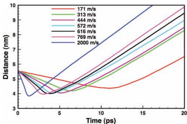
Figure 9. Plot of the distance of the center of mass of the monomer from the center of mass of the coated particle vs time. Each trajectory obtained has been averaged over all the reflected trajectories for a given incident speed.
