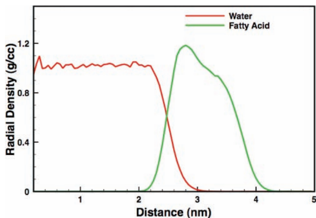
Figure 3. Radial density profiles of the coated particle. Distance is measured radially outward from the center of mass of the particle.
