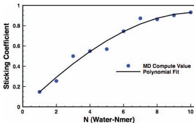
Figure 7. Sticking coefficients for water- N mers of different sizes for different values of N .
