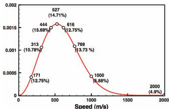
Figure 6. Sticking coefficients of the water monomer for various values of incident speeds on a Maxwell–Boltzmann speed distribution at 300 K. Percent values in parentheses are the fraction of sticking collisions at the given speed.
