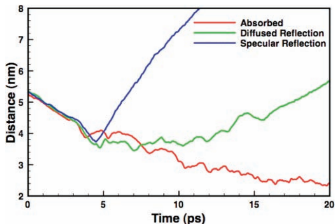
Figure 8. Distance of the center of mass of the incident monomer from the center of mass of the coated particle plotted as a function of time for the three types of interactions.
