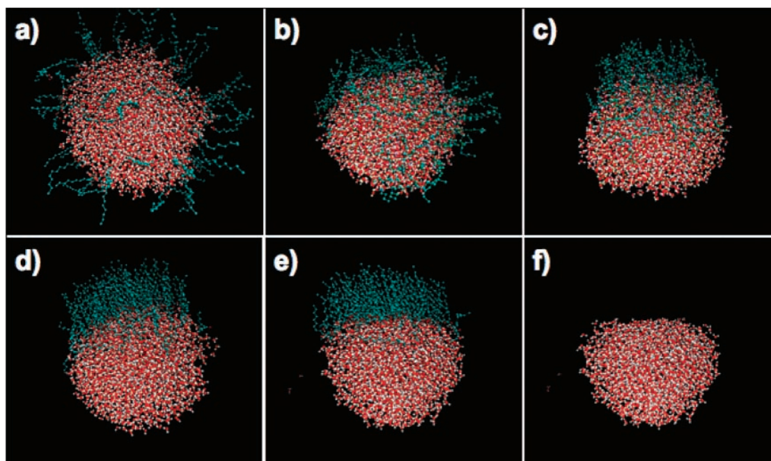
Figure 12. (a–e) Snapshots of the equilibration process of a particle consisting of 2440 water and 101 fatty acid molecules. (f) The snapshot of the final equilibrated structure without the fatty acid molecules (emphasizing the flat interface).
