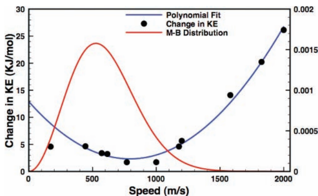
Figure 11. Change in KE is plotted for each incident speed case. The blue line is a polynomial (degree 2) fit to the change in KE data and is used to compute the average energy transferred per collision. Also plotted is the Maxwell–Boltzmann distribution for a water monomer at 300 K.
