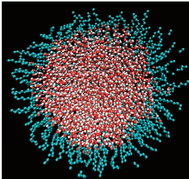
Figure 2. Cross-sectional view of an equilibrated coated particle at 260 K (consisting of 2440 water molecules and 505 fatty acid molecules).
