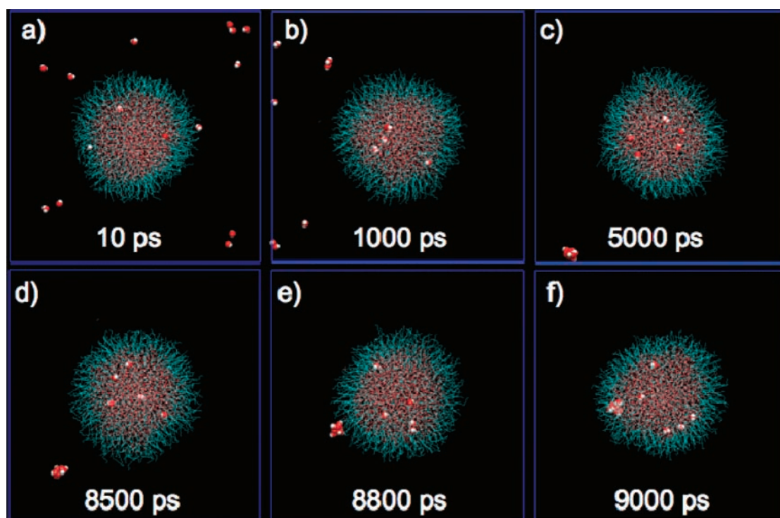
Figure 13. (Orthographic) snapshots of various stages of the 20 ns simulation to test the reduction in vapor pressure because of the coating. Larger spheres are used to represent the water molecules in the vapor phase.
