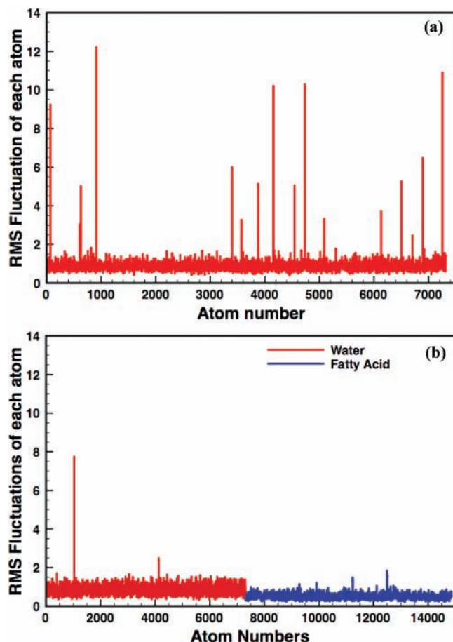
Figure 5. (a) Root-mean-square fluctuations of each atom in the pure water droplet resulting from heating. (b) Root-mean-square fluctuations of each atom in the coated droplet resulting from heating.
