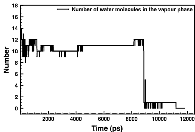
Figure 14. Plot of the number of water molecules in the vapor phase as a function of time.
