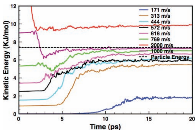
Figure 10. Plot of the change in kinetic energy (KE) of a monomer vs time. Each trajectory has been averaged over all the reflected trajectories for a given incident speed. The “dashed” line represents the thermal energy of the coated particle.
