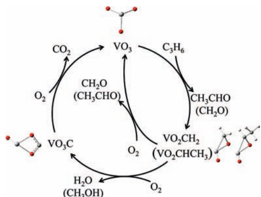
Figure 8. Schematic diagram showing barrierless reaction channels that form catalytic cycles for propylene (C 3 H 6 ) partial oxidation over the VO 3 cluster under gas phase, room temperature conditions.
