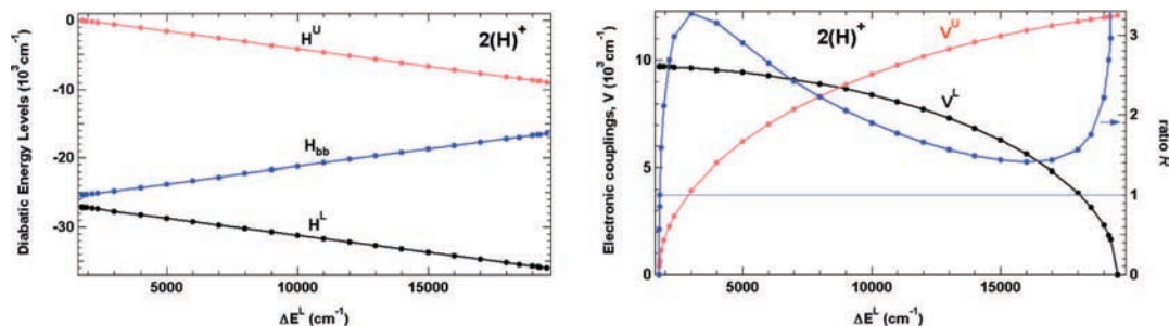
Figure 10. (Left panel) Plot of the diabatic energies of 22/Ph + obtained in a neighboring orbital analysis as a function of \Delta E^L . (Right panel) plot of the N.O. electronic couplings (left axis) and their ratio R = V^L/V^U as a function of \Delta E^L .
