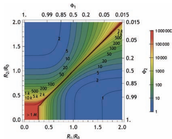
Figure 15. Contours of constant photon number as labeled on the figure that give \mathcal{S}(S,O) equivalent to 95% likelihood of distinguishing two states at FRET distances of R_1/R_0 and R_2/R_0 . The contours above the diagonal include only the intensity information whereas those below the diagonal include both the interphoton time and the sojourn time information. Plot was generated for k_{rd} = 1/(10 \text{ ns}) , k_{nra} = k_{nr} = 1/(100 \text{ ns}) , k_{ra} = 1/(2 \text{ ns}) , (S_i) = 1/2 , w = 100 \text{ ps} , \gamma = 10 , \beta = 1 , \xi = \delta = \epsilon = 0 .
