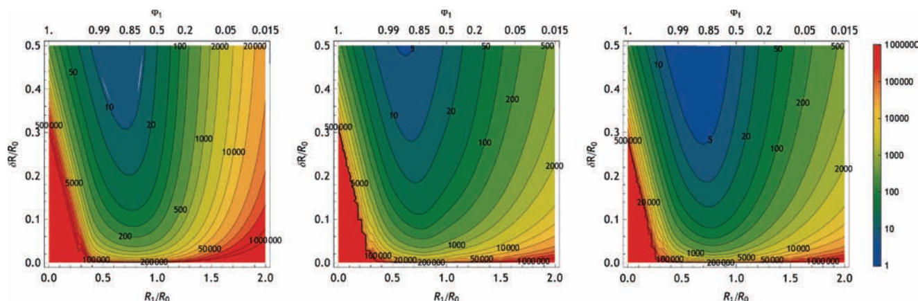
Figure 16. Contours of constant photon number as labeled on the figure that give \mathcal{I}(S, O) equivalent to 95% likelihood of distinguishing two states at FRET distances of R_1/R_0 and (R_1 + \delta R)/R_0 . The left panel shows the contribution from donor photons, the center panel shows the contribution from acceptor photons, and the right panel shows contributions from both. Experimental parameters are the same as in Figure 15.
