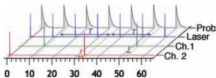
Figure 1. Basic concept of time-correlated single photon counting. Blue trace represent the intensity of the laser excitation pulses. Green and red traces represent the arrival of photons at different detectors that are resolved using a dichroic mirror. Gray decay functions represent the probability density for photon emission. t is the excited-state sojourn time (microtime) controlled by the lifetime, and T is the interphoton time (macrotime) related to the total emission intensity. An information theoretical analysis of two-channel macrotime measurements has been previously published. 1
