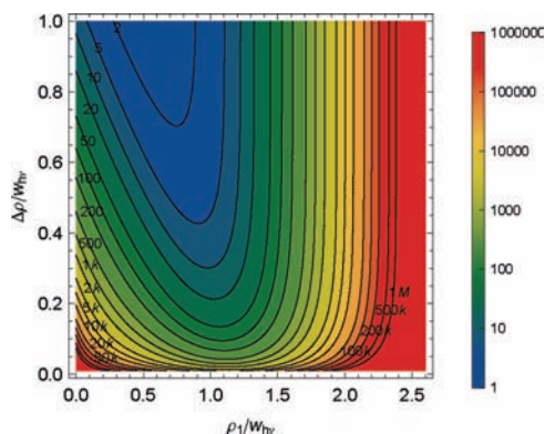
Figure 17. Contours of constant photon number as labeled on the figure that give \mathcal{I}(S, O) equivalent to 95% likelihood of distinguishing two positions in a Gaussian excitation beam. The contours above the diagonal include the effects of a 100 ps Gaussian instrument response whereas those below the diagonal include a 100 ps Gaussian IRF.
