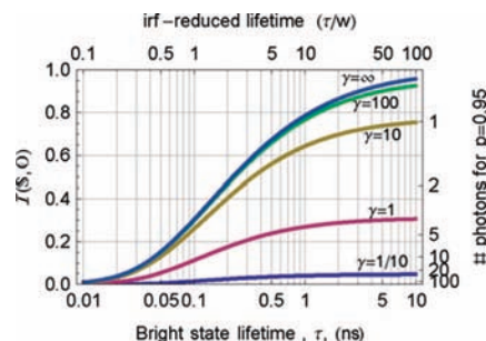
Figure 11. Mutual information between a dark state and a bright state as a function of bright-state lifetime for different levels \gamma = S:B of Raman-type background. The right axis shows the equivalent number of photons expected to distinguish the dark state at p = 0.95 .
