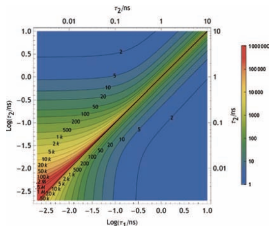
Figure 12. Contours of constant photon number as labeled on the figure that give \mathcal{S}(\text{S},\text{O}) equivalent to 95% likelihood of distinguishing two dyes (or states) with lifetimes \tau_1 and \tau_2 . The contours above the diagonal include the effects of a w = 1 ns Gaussian instrument response whereas those below the diagonal include a w = 100 ps Gaussian IRF. The green zone on the plot shows the ideal region for single molecule measurements.
