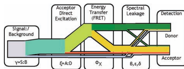
Figure 14. When cross-talk between channels is non-negligible, there are four contributions to the donor and acceptor channels: Directly excited acceptor emission, FRET acceptor emission, donor emission, and background. These contributions appear in eq 36.
