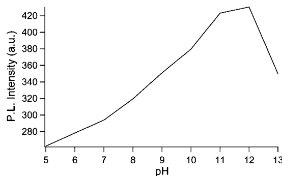
Figure 5. Change of PL intensity of ZnS:Cu,Cl colloidal NCs as a function of pH of the aqueous colloidal solution.
