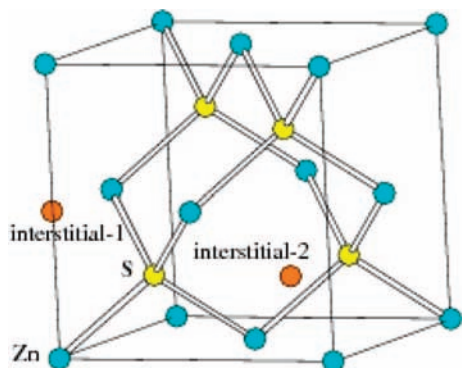
Figure 13. A cubic unit cell of zinc blende, illustrating the two interstitial sites for Cu (orange). Blue and yellow are for Zn and S, respectively.
