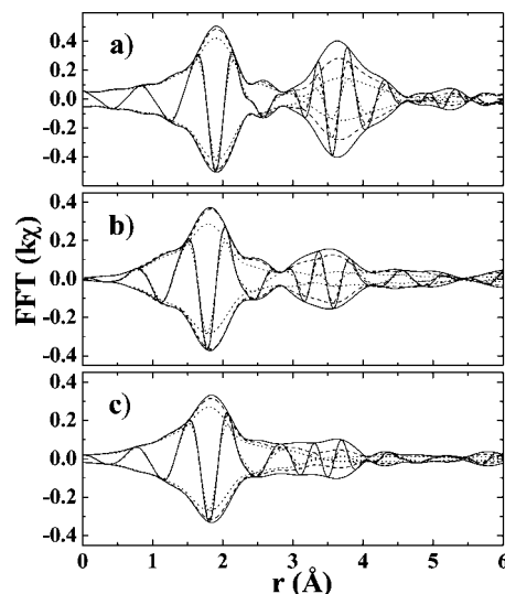
Figure 10. EXAFS r -space data for bulk material, at Cu and Zn K-edges. (a) Bulk ZnS:0.15%Cu,Cl, Zn K-edge, T = 4, 140, 300 \text{ K} ; (b) bulk ZnS:0.15%Cu,Cl, Cu K-edge, T = 4, 100, 300 \text{ K} ; and (c) bulk CuS reference, Cu K-edge, T = 4, 140, 300 \text{ K} . Here the fast oscillation is the real part of the transform; k -range is 3.5\text{--}11 \text{ \AA}^{-1} for Cu K-edge and 3.5\text{--}14 \text{ \AA}^{-1} for Zn K-edge; window Gaussian broadened by 0.3 \text{ \AA}^{-1} .
