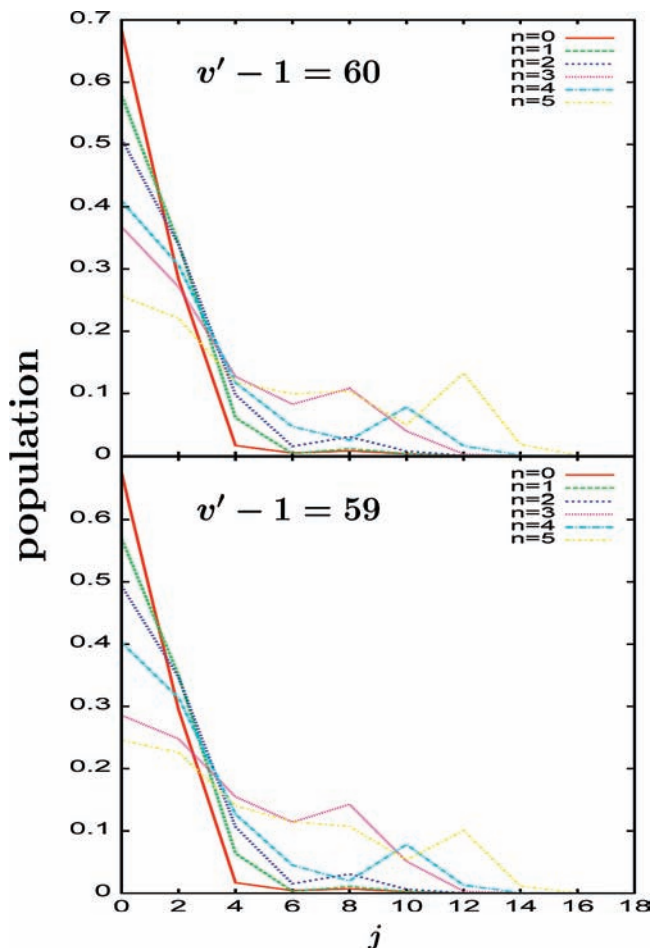
Figure 4. Free-rotor distributions associated with the wave functions of the six identified continuum resonances of v' - 1 = 60 (upper panel) and v' - 1 = 59 (lower panel). All of the distributions are normalized to unity.
