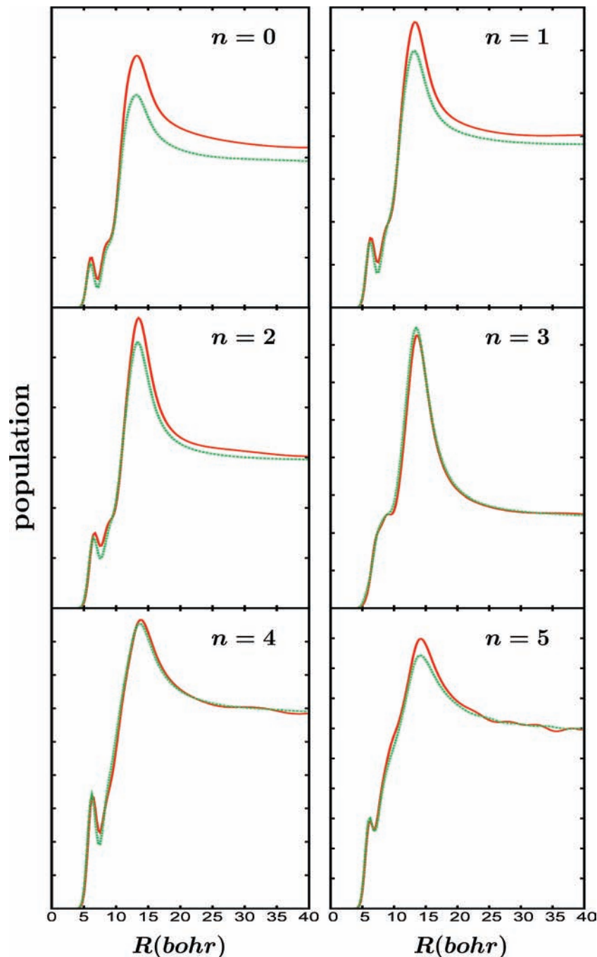
Figure 6. Comparison of the radial distributions associated with the wave functions of the v' - 1 = 60 (red solid lines) and v' - 1 = 59 (green dashed lines) continuum resonances.
