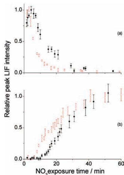
Figure 3. Intensity of LIF signals for (a) OD and (b) OH from reaction of O( 3 P) with a C 6 D 13 -SAM as a function of NO 2 exposure time. NO 2 pressures of 2 mTorr (black filled circles) and 6 mTorr (red open circles). Each point represents the peak height (with background subtracted) from a measured appearance profile. Data were recorded on the OD/OH A-X (1,0) Q 1 (1) line at a probe laser-SAM distance of 4 mm. Relative intensities for OH and OD at both pressures have been arbitrarily normalized to the peak signals at long and short exposure times, respectively.
