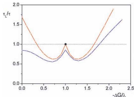
Figure 2. Free energy dependence of \tau_L/\tau calculated numerically at \lambda = 0.86 eV (solid lines). The blue and red lines correspond to the reversible and irreversible transfer, respectively. The symbol ● points to the result of ref 18.
