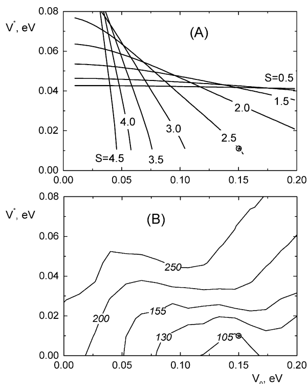
Figure 4. (A) Family of curves satisfying the condition k_0 = \langle W_l \rangle = 530 \text{ \AA}^3/\text{ps} at different S . (B) Contour map of k_2 values calculated along the curves shown in A. Symbol star-in-circle on both plots shows the point with k_0 and k_2 closest to those established for Per/TCNE system in eq 2.21. This point coordinates provide the microscopic ionization parameters V , V^* , S (eq 2.22).
