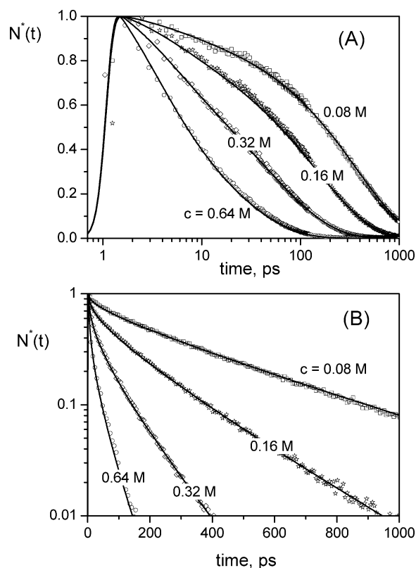
Figure 5. (A) Fitting the whole ionization kinetics at different concentrations with a double-channel rate W_l(r) ( V_0 = 0.15 \text{ eV} , V^* = 0.01 \text{ eV} , S = 2.5 , L = 1.24 \text{ \AA} ) and diffusion coefficient D = 260 \text{ \AA}^2/\text{ns} . (B) The same in the semilogarithmic scale showing the long time N^*(t) asymptotes.
