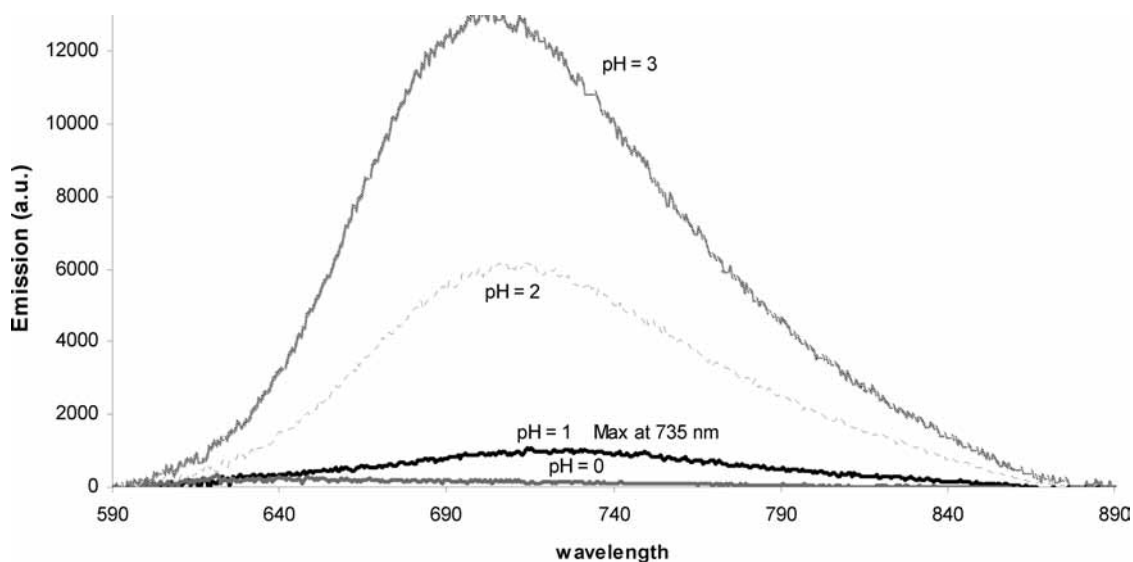
Figure 4. Emission spectra of Ru(bpy) 2 (dpp) 2+ at low pH. The red shift becomes discernible at pH 2, and the maximum shifts to 735 nm at pH 1.
