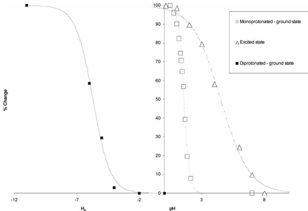
Figure 7. Ground- and excited-state titration curves for \text{Ru}(\text{bpy})_2(\text{dpp})^{2+} . From left to right, the curves correspond to diprotonation ( \blacksquare ) of \text{Ru}(\text{bpy})_2(\text{dpp})^{2+} , monoprotection of \text{Ru}(\text{bpy})_2(\text{dpp})^{2+} ( \square ), and protonation of the excited complex ( \triangle ) derived from UV-vis, NMR, and emission quenching, respectively.
