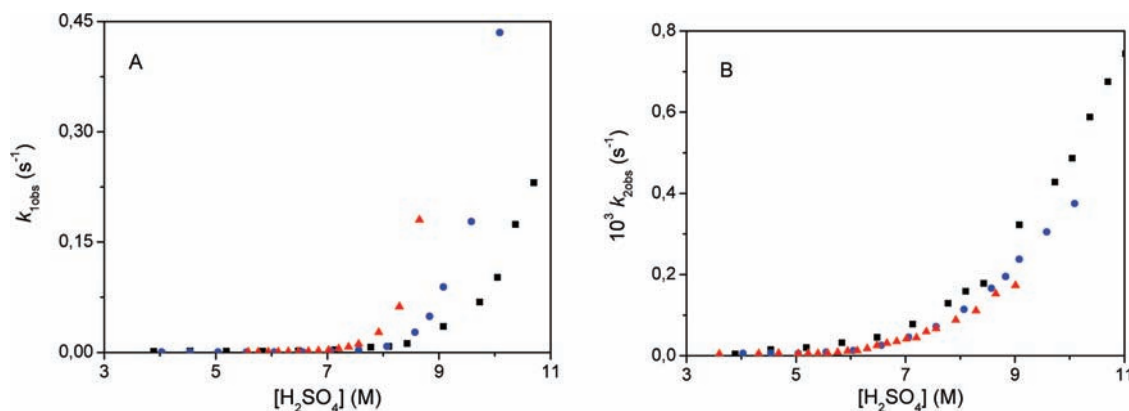
Figure 5. Plots of pseudo-first-order rate constants k_{1\text{obs}} (A) and k_{2\text{obs}} (B) vs molar sulfuric acid concentration for the hydrolysis of [\text{Pd}(\text{CNN})\text{P}(\text{OMe})_3]^+ at 25 °C: (□) 10% (v/v) ethanol–water; (●) 30% (v/v) ethanol–water; (▲) 50% (v/v) ethanol–water.
