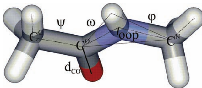
Figure 1. The N -methylacetamide molecule and selected geometry parameters: CO bond length ( d_{CO} ), the \psi ( \angle HCC^ON ), \omega ( \angle C^ONC^N ), and \phi ( \angle O^NCH ) dihedral angles, and the out-of-plane deviation (oop) of the nitrogen atom.
