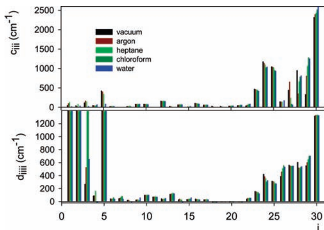
Figure 6. Diagonal cubic ( c_{iii} ) and quartic ( d_{iiii} ) normal mode constants for NMA calculated at the MP2/6-311++G**/CPCM level for different solvents.
