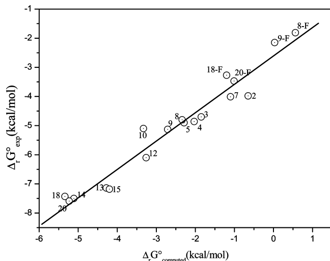
Figure 2. Correlation between \Delta_r G_{\text{DNP}}^{\circ}(\text{soln}) and \Delta_r G_{\text{DNP}}^{\circ}(\text{computed}) at B3LYP/6-311++G(3df,2p)//B3LYP/6-311+G(d) for all the studied compounds.
