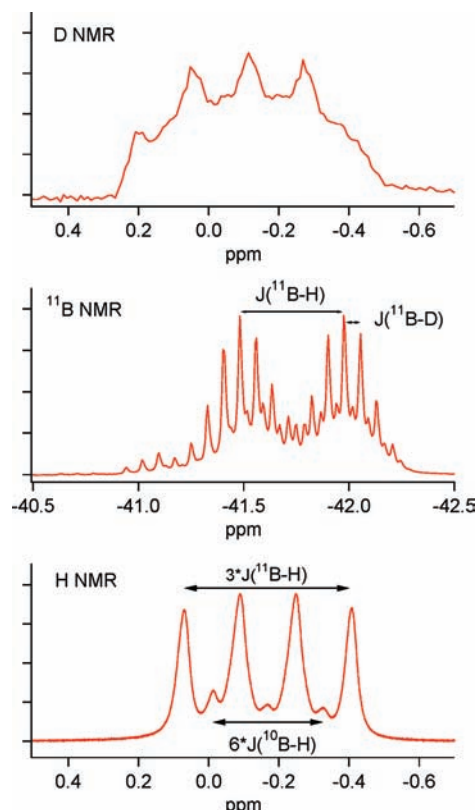
Figure 2. NMR spectra of NaBD 3 H in 1 M NaOD/D 2 O solution at room temperature.
