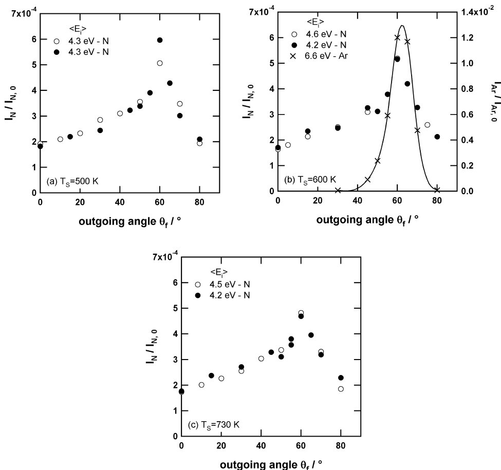
Figure 2. Angle-resolved density distributions of N atoms ( \langle E_f \rangle \sim 4.3 eV; open and filled circles) and Ar atoms ( \langle E_f \rangle \sim 6.6 eV; crosses) scattered from Ag(111) at \theta_i = 60^\circ . The panels show (a) N, T_S = 500 K; (b) N and Ar, T_S = 600 K; and (c) N, T_S = 730 K. The scattered Ar intensities in (b) are indicated on the right ordinate. The scattered intensities are normalized to the intensity of the corresponding direct beam. For all three surface temperatures, two independent data set are plotted for the N density distributions. The line connecting the Ar points is intended to guide the eye.
