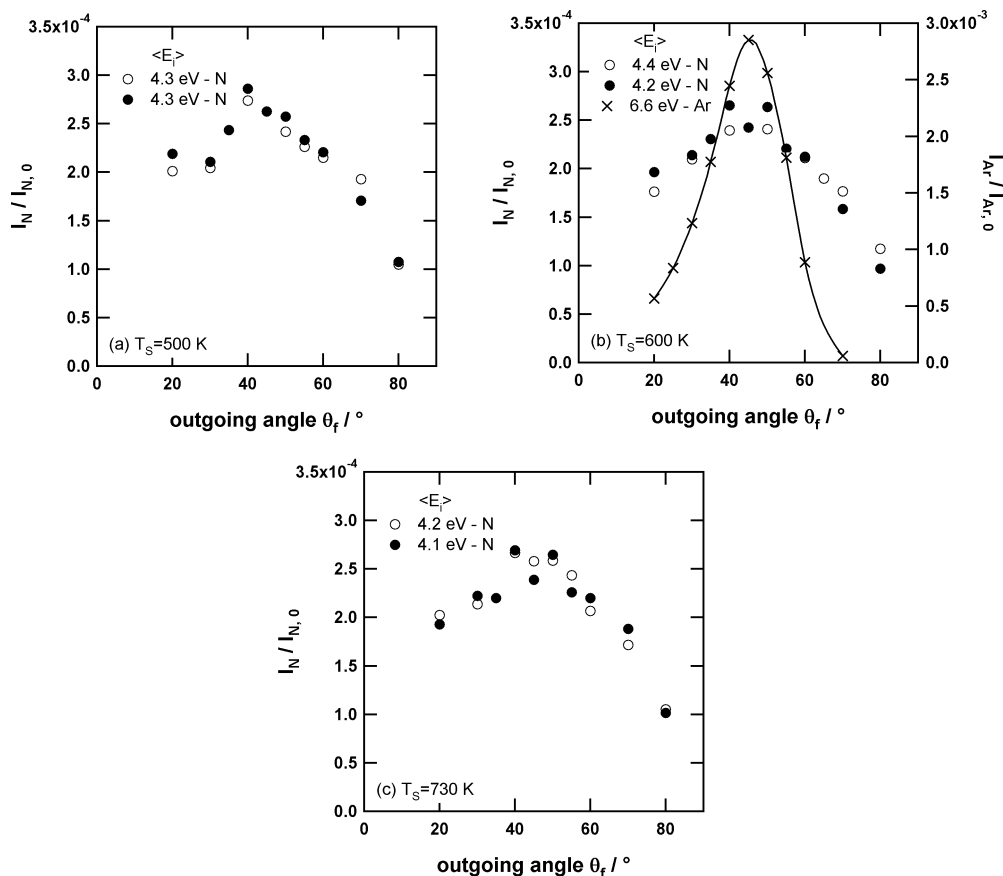
Figure 1. Angle-resolved density distributions of N atoms ( \langle E_i \rangle \sim 4.3 eV; open and filled circles) and Ar atoms ( \langle E_i \rangle \sim 6.6 eV; crosses) scattered from Ag(111) at \theta_i = 40^\circ . The panels show (a) N, T_S = 500 K; (b) N and Ar, T_S = 600 K; and (c) N, T_S = 730 K. The scattered Ar intensities in (b) are indicated on the right ordinate. The scattered intensities are normalized to the intensity of the corresponding direct beam. For all three surface temperatures, two independent data set are plotted for the N density distributions. The line connecting the Ar points is intended to guide the eye.
