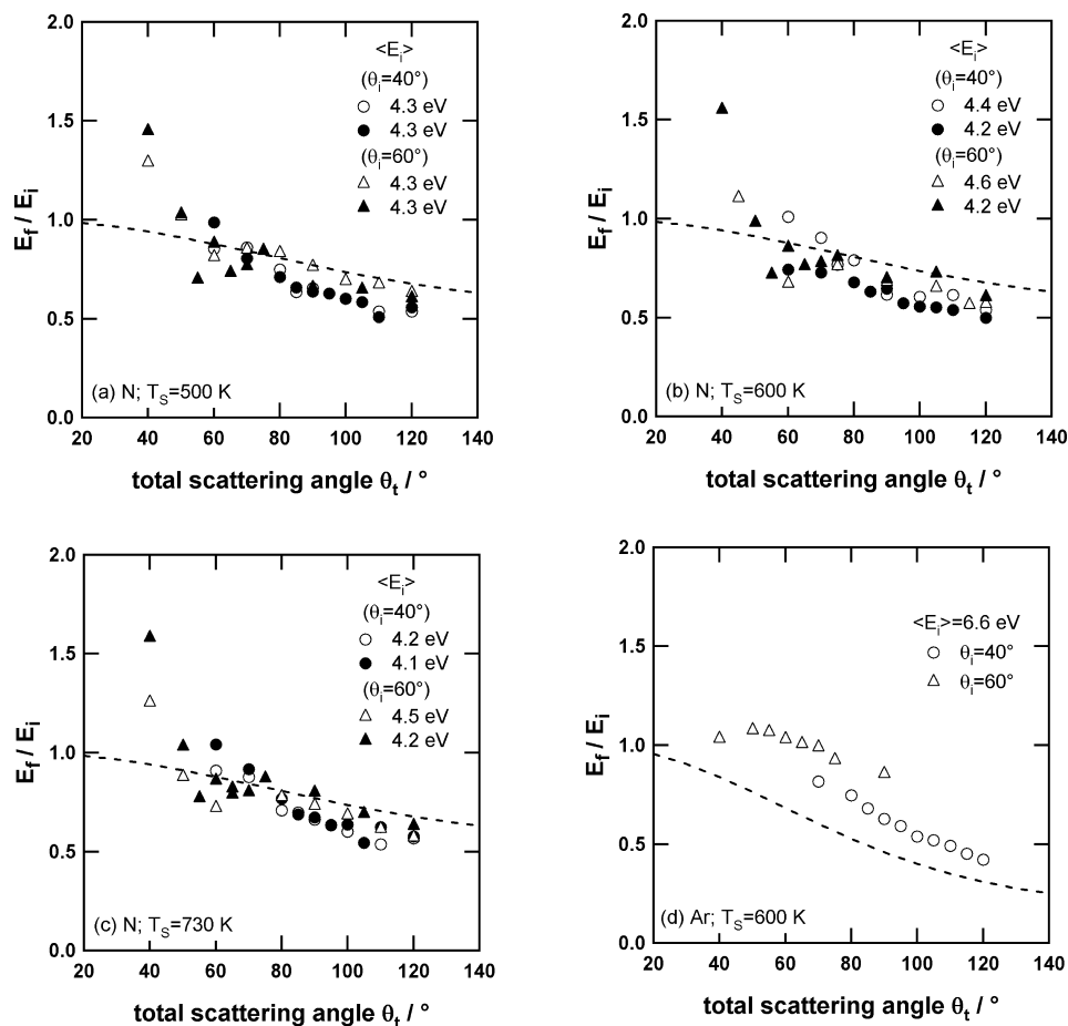
Figure 3. Angle-resolved ratios of final to initial energy ( E_f/E_i ) plotted as a function of the total scattering angle ( \theta_t = 180 - (\theta_i + \theta_f) ) for N atoms ( \langle E_i \rangle \sim 4.3 eV) scattered from Ag(111) at (a) T_s = 500 K, (b) T_s = 600 K, and (c) T_s = 730 K. (d) shows E_f/E_i for Ar atoms ( \langle E_i \rangle \sim 6.6 eV) scattered from Ag(111) at T_s = 600 K. Data sets are shown for \theta_i = 40^\circ (circles) and \theta_i = 60^\circ (triangles). Duplicate determinations (open and filled symbols) are shown for N atom scattering. The dashed lines represent the model of single-collision hard-sphere scattering of the incident atoms from an isolated silver “atom” (mass ratios of m_N/M_{Ag} = 14/108 and m_{Ar}/M_{Ag} = 40/108 , respectively).
