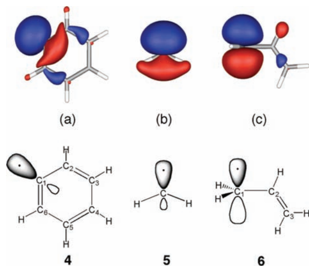
Figure 5. \sigma SOMOs of (a) phenyl radical ( 4 ), (b) triplet methylene ( 5 ), and (c) an allyl radical ( 6 ), but with the radical center at C(1) twisted out of conjugation and constrained to be locally planar. The orbital plots were made with an isodensity value of 0.015.
