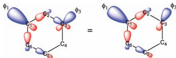
Figure 6. Schematic depiction of the AOs that make major contributions to the GVB orbital of 1 that is comprised largely of \phi_1 on C(1). \phi_3 at C(3) interacts through space with \phi_1 . The AOs at C(2) and C(6) that interact with the smaller lobe of \phi_1 are analogous to the 1s AOs on H that are found in the 3a_1 MO of any bent AH_2 molecule. The AOs at C(3) and C(5) that are parallel to the AO at C(1) come from hyperconjugative interactions of \phi_1 with the C(2)–C(3) and C(5)–C(6) \sigma and \sigma^* bonds. The two AOs at C(3) mix to give a resultant AO, \phi_3' , that is rotated more toward C(1) than \phi_3 is.
