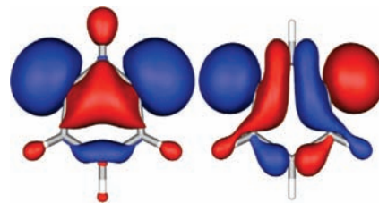
Figure 4. TCSCF orbitals, \psi'_S and \psi'_A of 1 plotted with an isodensity value of 0.030. The TCSCF MOs are, respectively, the sum and difference of the GVB orbitals in Figure 2.
