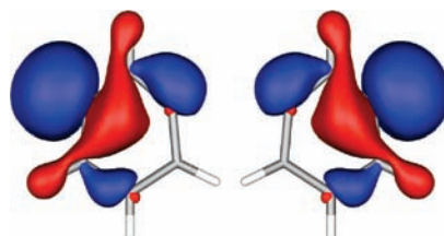
Figure 2. Pair of fully delocalized GVB orbitals for 1,3-dehydrobenzene ( 1 ), plotted with an isodensity value of 0.030. Basis functions on all the atoms were allowed to contribute to each of the GVB orbitals, so that both TS and TB interactions were incorporated into the GVB wave function.
