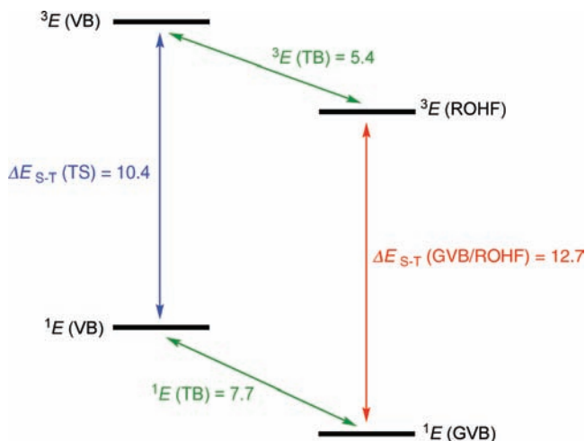
Figure 3. Results of triplet and singlet VB, triplet ROHF, and singlet GVB calculations on 1 with the 6-31G(d) basis set at ROHF and GVB/6-31G(d) optimized geometries. Energy differences are adiabatic and are given in kcal/mol. A Figure showing the relationship between the adiabatic and the vertical energy differences at the GVB/6-31G(d) optimized geometry is available in the Supporting Information. 17
