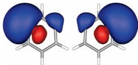
Figure 1. Pair of semilocalized VB orbitals for 1,3-dehydrobenzene ( 1 ), plotted with an isodensity value of 0.015. Only basis functions on C(1) and C(3) were allowed to contribute to each of the VB orbitals. Therefore, TS but not TB interactions between these two carbons is incorporated into the VB wave function.
