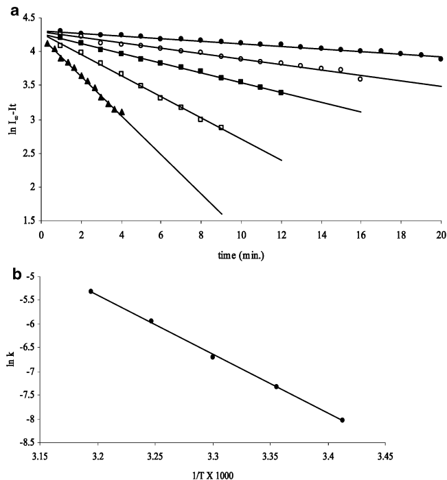
Figure 7. (a) Rate constants of the formation of the \text{Ag}^+ -I complex at 20 (●), 25 (○), 30 (■), 35 (□), and 40 °C (▲) upon the addition of [\text{Ag}^+] = 1.0 \times 10^{-5} M to [\text{I}] = 1.0 \times 10^{-5} M at \lambda_{\text{ex}} = 333 nm, and \lambda_{\text{em}} = 488 nm. (b) Arrhenius plot for the \text{Ag}^+ -I complex.
