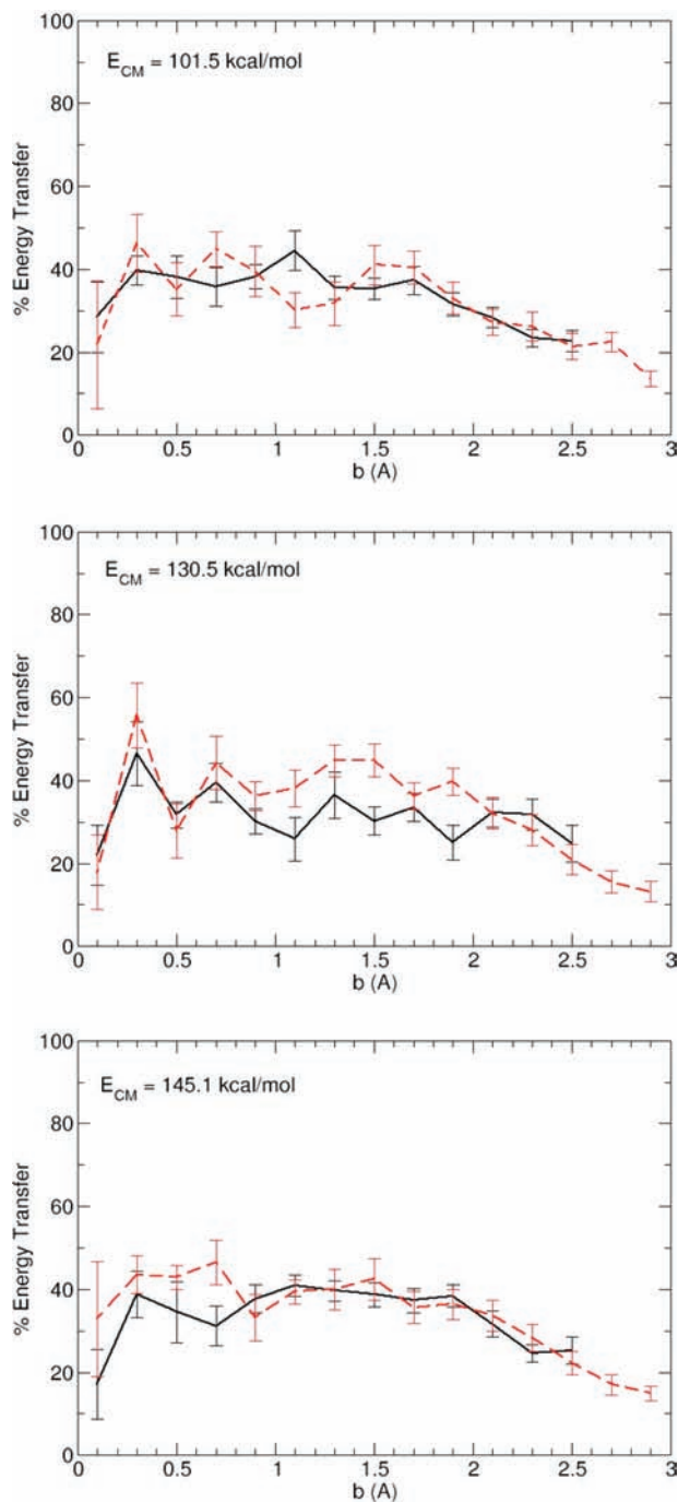
Figure 6. Percentage energy transfer to the internal degrees of freedom (vibration + rotation) of the two urea-H + isomers versus impact parameter for the three collision energies: OPr, solid line; NPr, dashed line. Uncertainties are standard deviation of the means.
