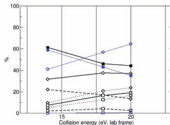
Figure 9. Percentages of remaining NPR reactant (■), NH 3 + CONH 2 + products for path 1 (□), and NH 4 + + OCNH products for path 2 (◇), for the three collision energies. Total percentage, (—); ET percentage, (---); shattering percentage, (···). In blue we show results obtained from kinetic analysis.
