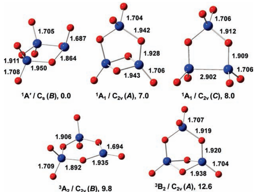
Figure 6. Low-lying electronic states of W_3O_8 calculated at the CCSD(T)/aVDZ//B3LYP/aVDZ level. Relative energies are given in kcal/mol.
