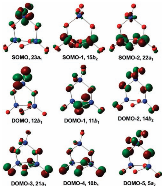
Figure 8. Singly occupied and highest few doubly occupied molecular orbitals (SOMOs and DOMOs) for the ground state of Cr_3O_8^- at the BP86/aVDZ level.
