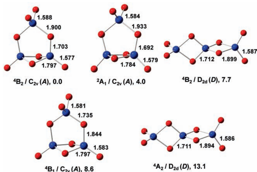
Figure 5. Low-lying electronic states of \text{Cr}_3\text{O}_8^- calculated at the CCSD(T)/aVDZ//B3LYP/aVDZ level. Relative energies are given in kcal/mol.
