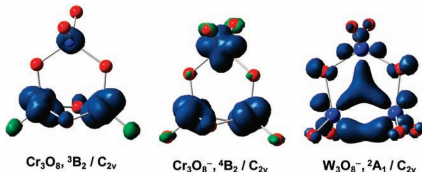
Figure 10. Electron spin density for the ground states of \text{Cr}_3\text{O}_8 , \text{Cr}_3\text{O}_8^- , and \text{W}_3\text{O}_8^- .
