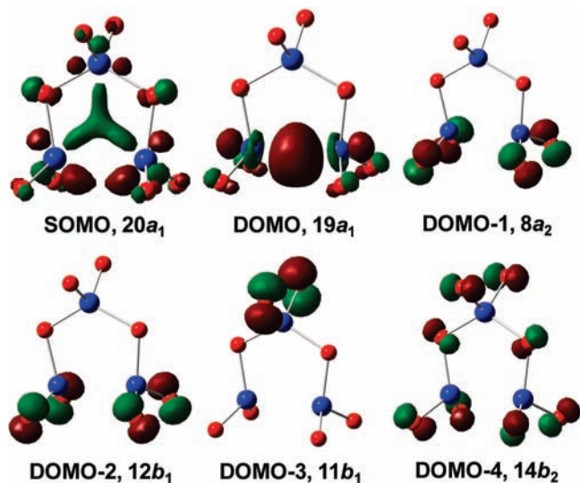
Figure 9. Singly occupied and highest few doubly occupied molecular orbitals (SOMOs and DOMOs) for the ground state of W_3O_8^- at the B3LYP/aVDZ level.
