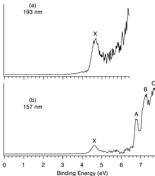
Figure 2. Photoelectron spectra of W_3O_8^- at (a) 193 nm and (b) 157 nm.
