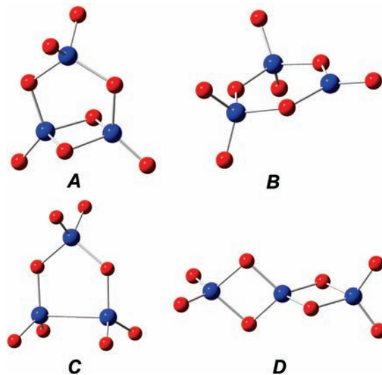
Figure 3. Molecular structures of the M_3O_8 and M_3O_8^- ( M = Cr, W ) clusters.
