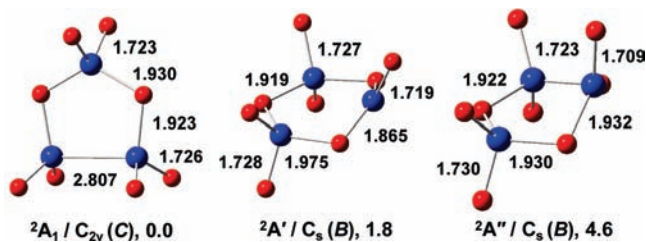
Figure 7. Low-lying electronic states of W_3O_8^- calculated at the CCSD(T)/aVDZ//B3LYP/aVDZ-PP level. Relative energies are given in kcal/mol.
