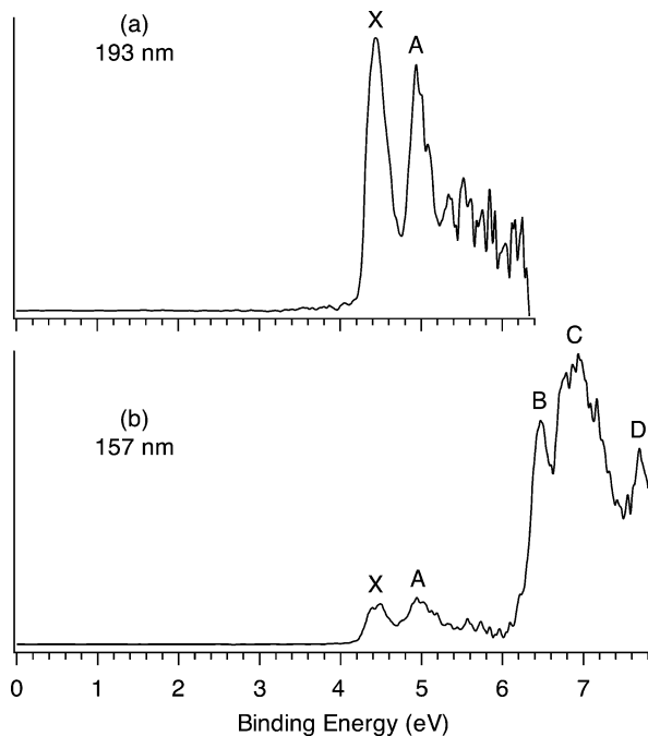
Figure 1. Photoelectron spectra of Cr_3O_8^- at (a) 193 nm (6.424 eV) and (b) 157 nm (7.866 eV).
