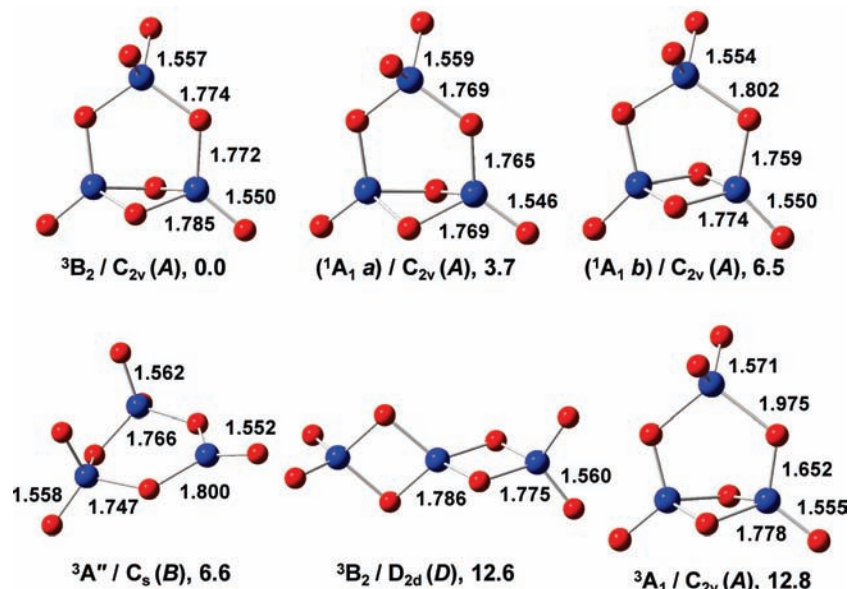
Figure 4. Low-lying electronic states of \text{Cr}_3\text{O}_8 calculated at the CCSD(T)/aVDZ//B3LYP/aVDZ level. Relative energies are given in kcal/mol.
