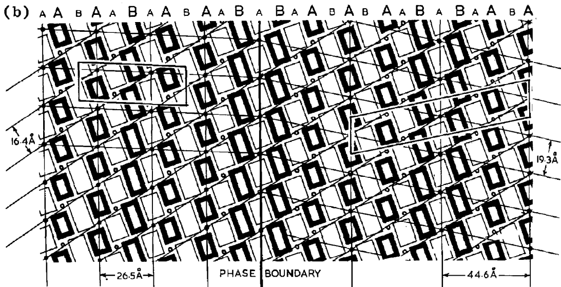
FIG. 3a. Lattice image of a crystal fragment with domains of \text{WNb}_{40}\text{O}_{103} at C and \text{WNb}_{68}\text{O}_{173} at D separated by a faulted region. Y is the different fringe sequence discussed in the text. The diffraction pattern of the fragment is inset. 3b. Idealized model of the region enclosed in the rectangle in Fig. 3a.
