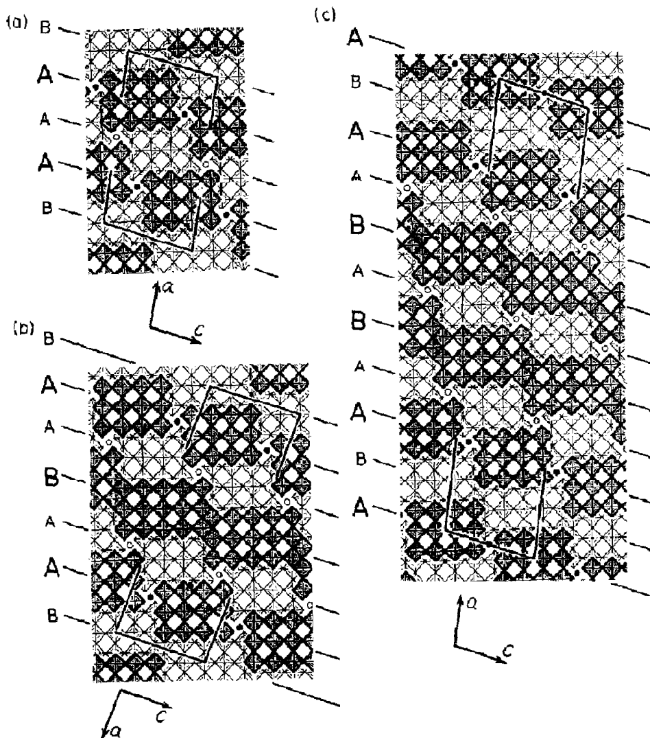
FIG. 5. Idealized models of the structures of the three new phases showing the row sequences. 5a. \text{WNb}_{24}\text{O}_{88} ; 5b. \text{WNb}_{40}\text{O}_{133} ; 5c. \text{WNb}_{68}\text{O}_{173} .
