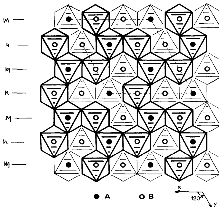
FIG. 4. The \text{Na}_2\text{SiF}_6 structure type.
