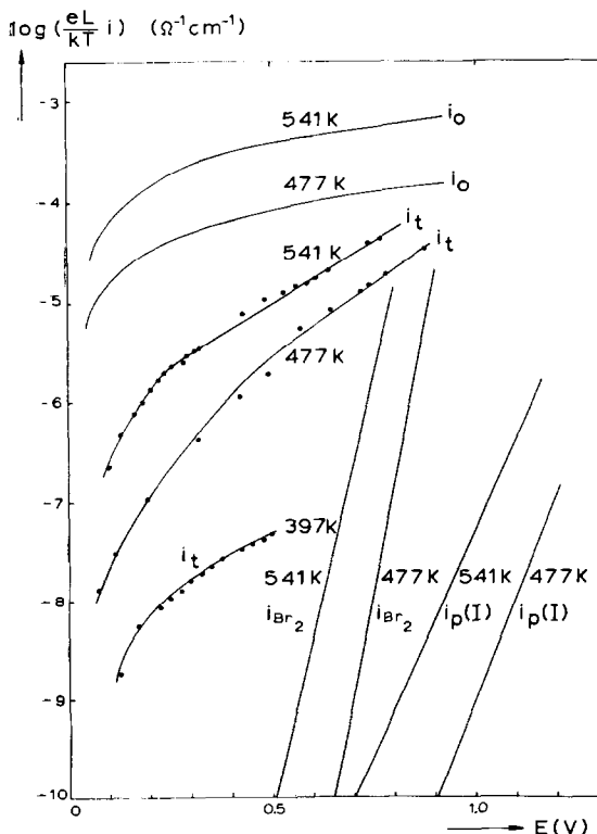
FIG. 1. The total current, i_t , the unblocked current, i_o , the decomposition current, i_{Br_2} , and the predicted hole current, i_p , in lead bromide, plotted as \log(eL/kT)i versus E .
