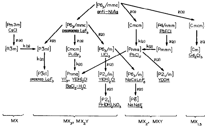
FIG. 1. Subgroup diagram of space groups derived from P6_3/mmc .
