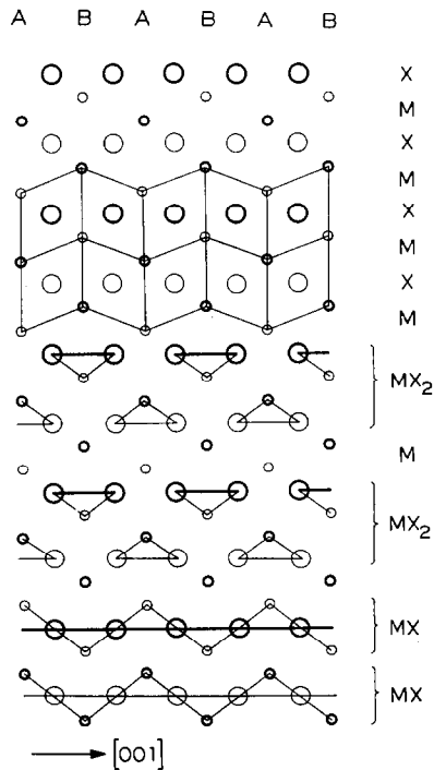
FIG. 2. The anti-NiAs-type structure projected on (11\bar{2}0) . Large and small circles represent, respectively, anions ( X or Y ) and cations ( M ). Heavy and light circles are at 0 and \frac{1}{3} along the projection axis, respectively.)
