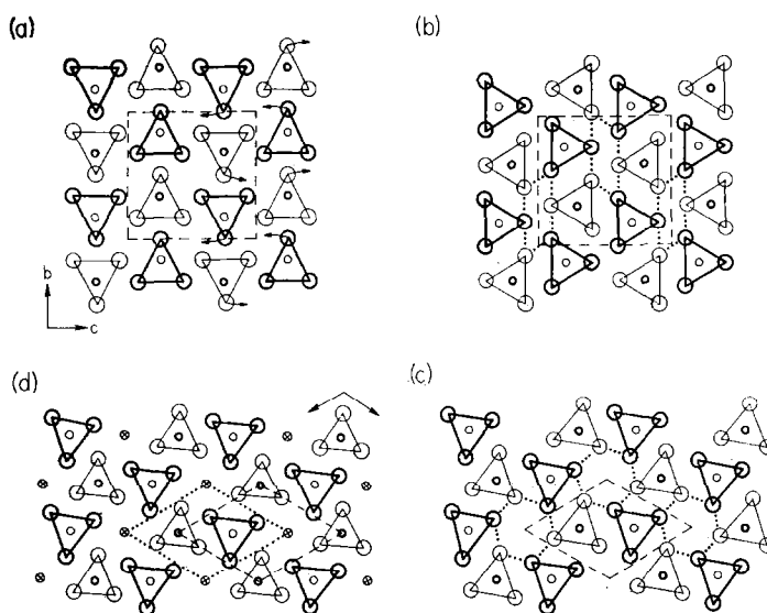
FIG. 5. The derivation of \text{UCl}_3 - and \text{NaNdF}_2 -type structures from disordered \text{LaF}_3 . (a) The structure of disordered \text{LaF}_3 (cf. Fig. 3c). (b) An intermediate structural arrangement obtained by distortion of \text{LaF}_3 . (c) The structure of hexagonal \text{UCl}_3 projected on (001). (d) The projection of hexagonal \text{NaNdF}_4 on (001). (The positions of Na ions ordered at z = 0.656 in one-half of the octahedral sites are shown by crossed circles. The projected \text{NaNdF}_4 cell is indicated by dashed lines; the equivalent cell which is coincident with that of \text{UCl}_3 is outlined by dots.)
