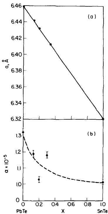
FIG. 2. (a) Lattice parameter at 0°C, a_0 , and (b) thermal expansion coefficient, \alpha , for the \text{Pb}_{1-x}\text{Sn}_x\text{Te} alloy system.
