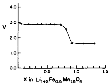
FIG. 7. Open-circuit voltage vs x for \text{Li}/1 M \text{LiClO}_4 \text{PC}/\text{Li}_{2+x}\text{FeMn}_3\text{O}_8 .
