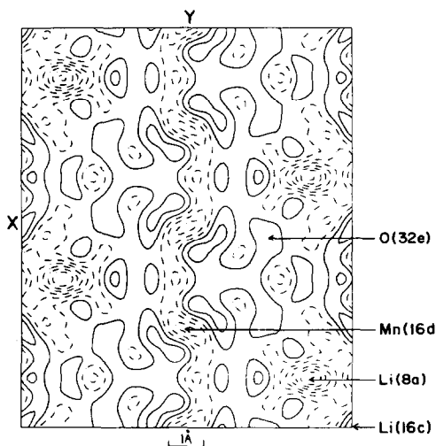
FIG. 3. The difference Fourier section of \text{Li}_2[\text{Mn}_2]\text{O}_4 (Model I) at height 0 perpendicular to [1 1 0] showing \text{Li}^+ occupation of both 8a and 16c sites of the spinel structure.
