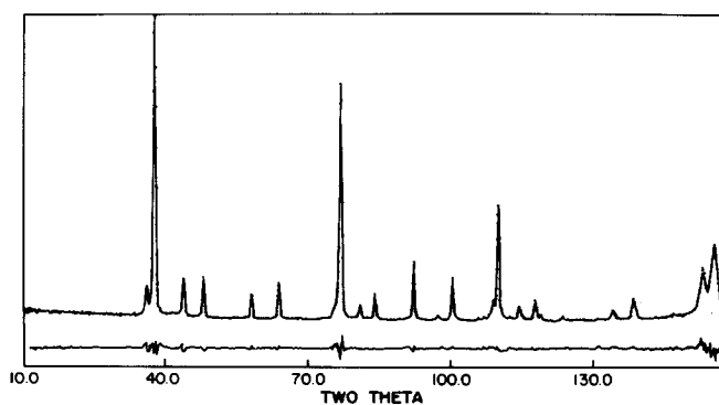
FIG. 5. The observed and calculated neutron diffraction powder patterns for \text{Li}_{0.2}[\text{Mn}_2]\text{O}_4 . The difference between the observed and calculated profiles is plotted below on the same scale.
