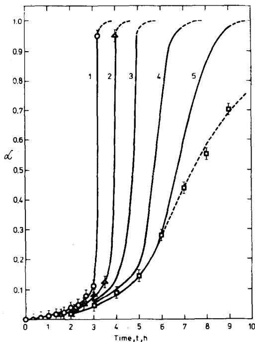
FIG. 2. Experimental and theoretical results of the SnS mechanochemical synthesis kinetics. Kinetic curves: curve 1, explosive mechanochemical synthesis of pure SnS; curve 2, explosive mechanochemical synthesis of SnS in the presence of 6% by weight of an inert admixture of \text{SiO}_2 ; curve 5, explosiveless mechanochemical synthesis of SnS in the presence of 12% by weight of an inert admixture of \text{SiO}_2 . Kinetic curves 3 and 4 are obtained under conditions intermediate between those for kinetic curves 2 and 5. Kinetic curve 3 is typical for an explosive mechanochemical synthesis, while kinetic curve 4 is typical for a smooth explosiveless mechanochemical synthesis.
