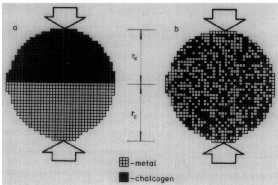
FIG. 1. Formation of mechanical aggregates with critical size r_c from metal and a chalcogen element: (a) aggregates typical for the initial state of dispersion (first stage of dispersion); (b) aggregates typical for the instant just before the mechanochemical explosion (second stage of dispersion).
