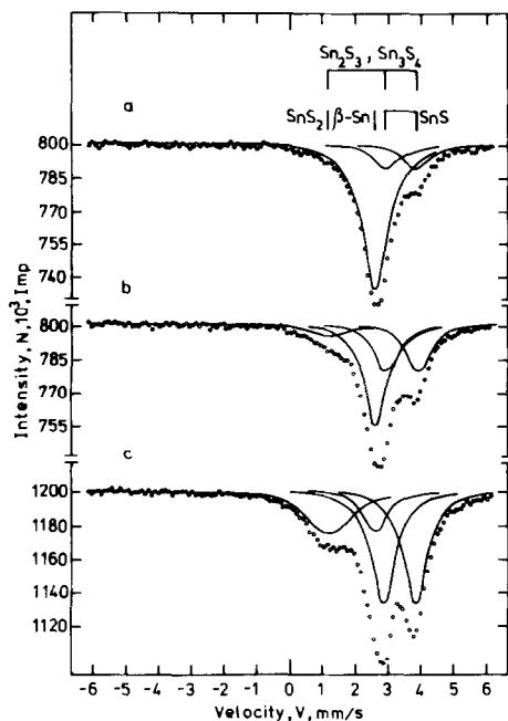
FIG. 3. Mössbauer spectra of samples from the explosiveless SnS mechanochemical synthesis in the presence of 12% by weight of an inert admixture of SiO 2 (kinetic curve 5, Fig. 2): (a) 4-hr mechanical activation; (b) 6-hr mechanical activation; (c) 9-hr mechanical activation.
