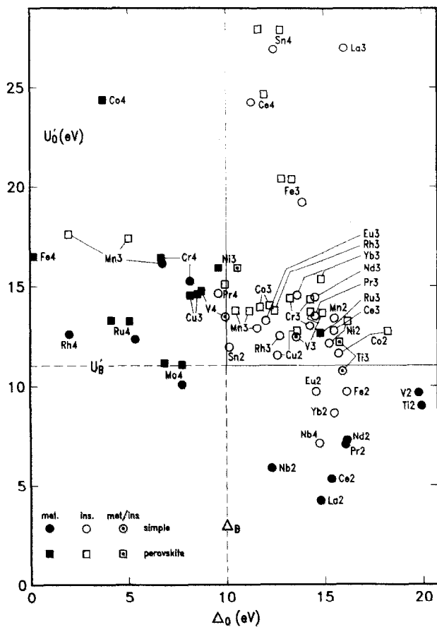
FIG. 2. A plot of the calculated values of U_0 and \Delta_0 for the 76 oxides in Table I. The lines attempt to separate the "insulators" (open symbols) from the "metals" (solid symbols) according to the ZSA framework.
