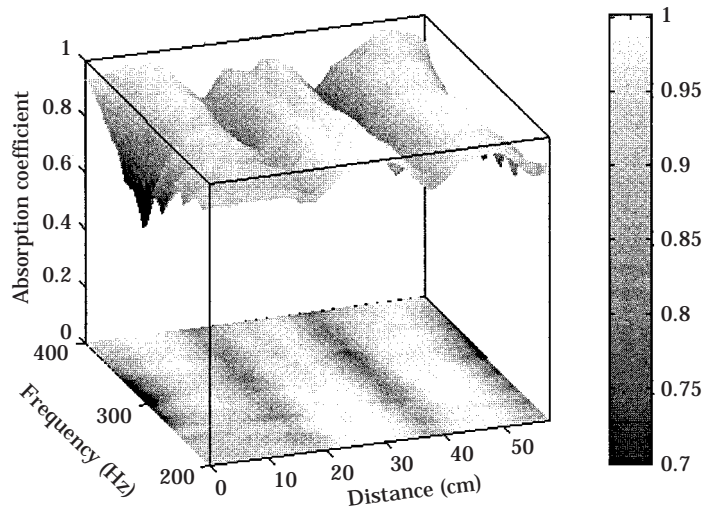
Figure 20. Absorption coefficient of the fibreglass panel backed by a 3 \times 3 loudspeakers array under normal incidence.
