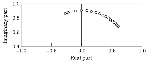
Figure 12. Floquet multiplier with collocation periodic solution; P = 1.1 , D = 0.03 , G = 0.03 , \Omega = 1 , \alpha = 0.16 , F = 0.02-2 .
