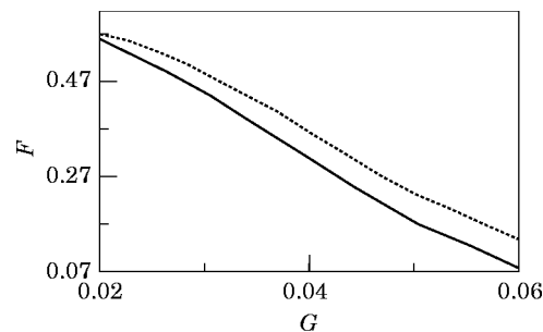
Figure 9. Stable period-1, period-2, and unstable regions; P = 1.1 , D = 0.03 , \Omega = 1 , \alpha = 0.05 ; —, P-1-P-2 ; ----, P-2 -unstable.
