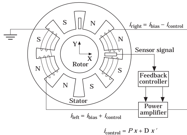
Figure 1. Rotor magnetic bearing system.
