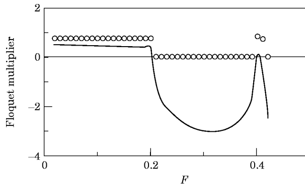
Figure 7. Period-doubling bifurcation; P = 1.1 , D = 0.03 , G = 0.03 , \Omega = 1 , \alpha = 0.16 . Key as for Figure 6.
