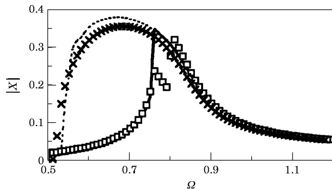
Figure 3. Non-linear frequency response; P = 3, D = 0.11, E = 0.03, \alpha = G = 0 . Key: \square , TCM increasing speed; \times , TCM decreasing speed; — , RK increasing speed; --- , RK decreasing speed.
