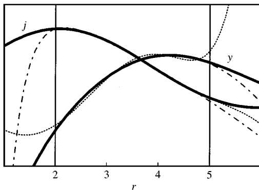
Figure 3. A demonstration showing why inverse powers are required in the fitting of the second kind of spherical Bessel function. Thick lines are j_{1.5}(r) and y_{1.5}(r) . The fitted interval is 2 < r < 5 . The dash-dotted lines are the resultant polynomial functions in terms of the set of \{r^{-3}, r^{-1}, r^1, r^3\} , while the dotted lines are \{r, r^3, r^5, r^7\} . We can see that the set of \{r, r^3, r^5, r^7\} is not suitable to fit y_{1.5}(r) accurately, while the set of \{r^{-3}, r^{-1}, r^1, r^3\} gives reasonable fitting both for j and y functions.
