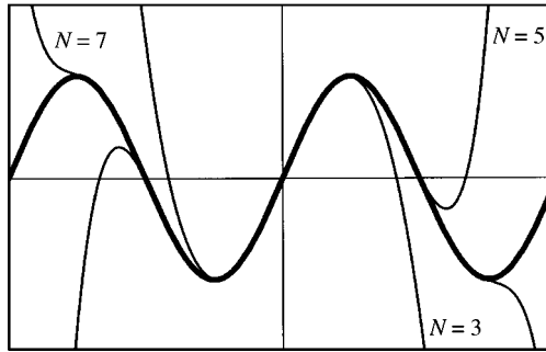
Figure 1. An example showing how a sinusoidal function is fitted well by power functions. Note that odd powers \{x, x^3, x^5, x^7\} were used in the fitting because the sine function (thick line) is an odd function. Thin lines are the resultant polynomial functions after fitting; N is the maximum power used in the fitting. For instance, N = 5 specifies that the set of \{x, x^3, x^5\} are used in the fitting. We can see that the fittable range increases with increasing N .
