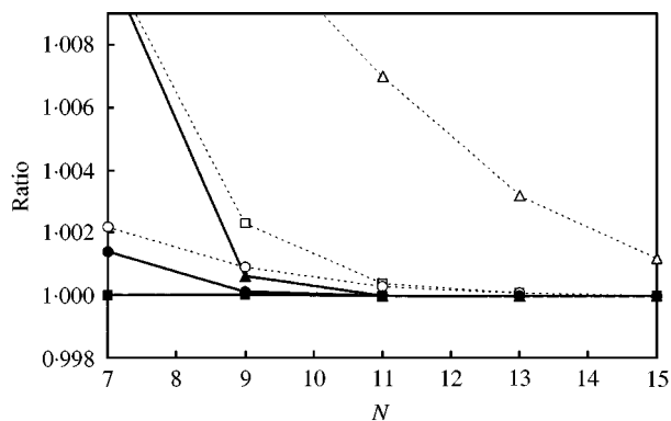
Figure 5. Comparison of convergency between the xyz (dotted lines with open symbols) and the xyzr (solid lines with solid symbols) algorithms for some selected modes. The data in Table 2 are used. Note that k is chosen to be \sim N/2 for the xyzr algorithm: --\square-- {}_0S_0 ; ---\triangle--- {}_0S_2 ; -\circ- {}_0T_2 .
