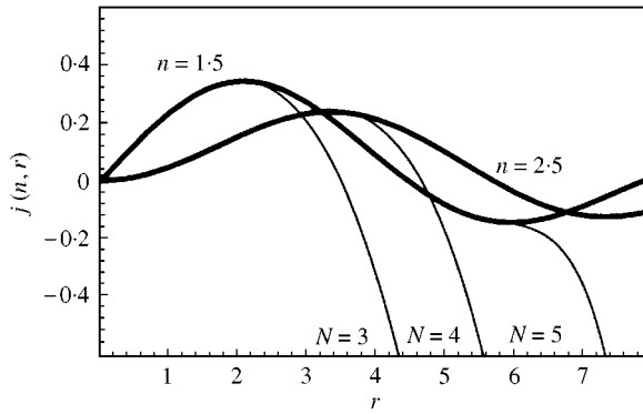
Figure 2. An example showing how the first kind of spherical Bessel function is fitted well by power functions. Thick lines are j_{1.5}(r) and j_{2.5}(r) , in the displacement functions of {}_qS_0 and {}_0T_n , respectively. Procedures are similar to that in Figure 1. Note that N = 3, 4, and 5 specify the set of power functions used, or \{r^1, r^3\} , \{r^0, r^2, r^4\} , and \{r^1, r^3, r^5\} respectively.
