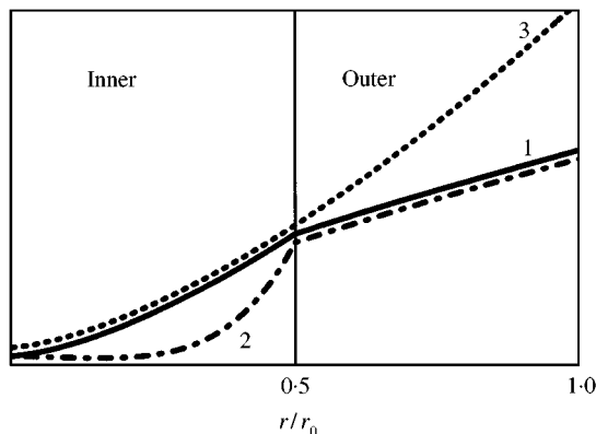
Figure 4. Schematic illustration of various base functions. The numbers correspond to those defined in equations (6)–(8).
