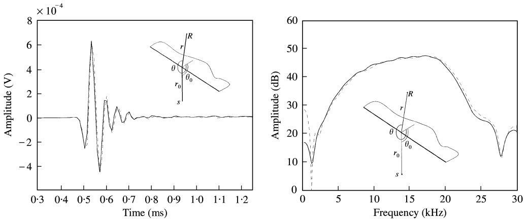
Figure 5. Same as Figure 4 but for r_0 = 10.0 cm, \theta_0 = 88.5^\circ , r = 13.9 cm, \theta = 271.5^\circ .
