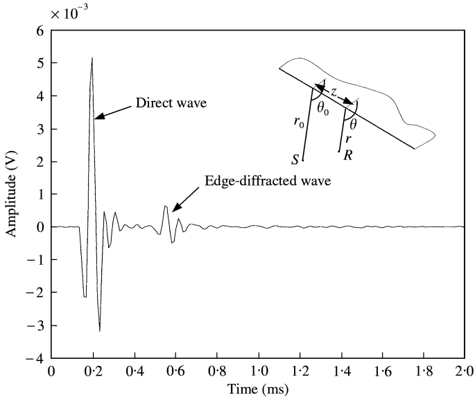
Figure 3. Experimental determination of the impulse response for a thin metallic plane in the incidence zone. r_0 = 8.9 cm, \theta_0 = 92^\circ , r = 6.9 cm, \theta = 91.6^\circ , z = 2.6 cm.
