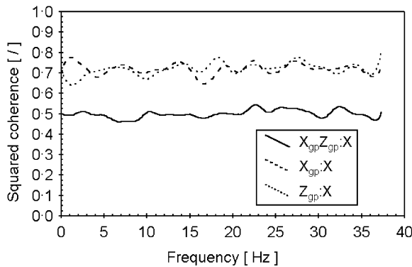
Figure 12. Multiple coherence.
