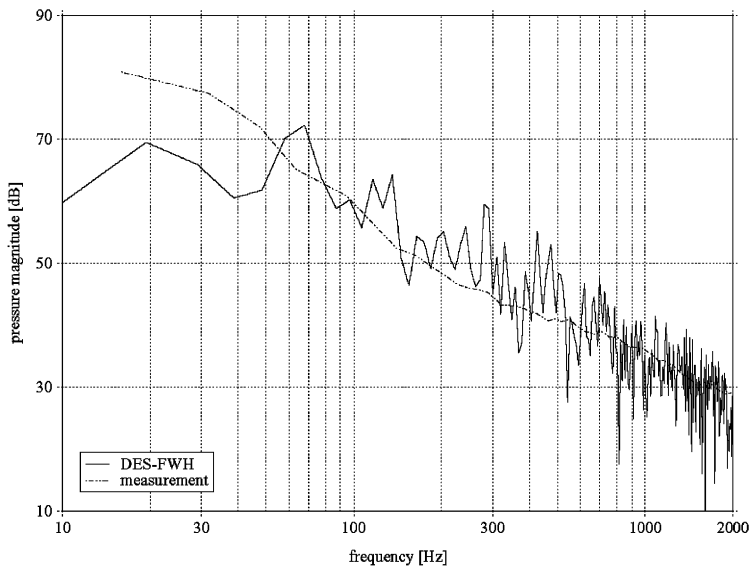
Figure 8. Measured and calculated sound spectra at a selected position.
