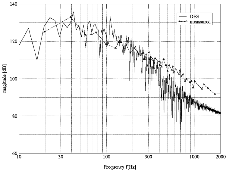
Figure 7. Measured and calculated surface pressure spectra at a selected sensor location based on DES.
