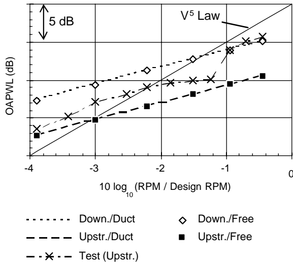
(b) Overall sound power level versus rotation speed
