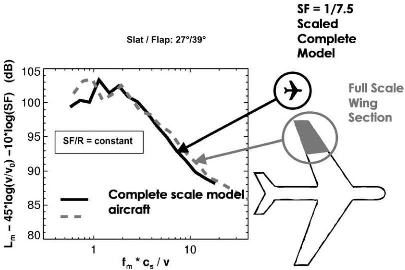
Figure 4. Comparison of non-dimensional wing high-lift farfield slat noise spectra from 1/7.5 model- and full-scale wind tunnel experiments.
