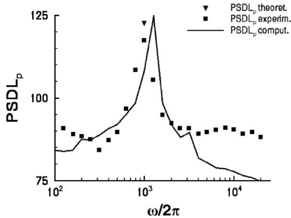
Figure 9. Third-octave spectrum of the sound emission of an unsteady flow around a circular cylinder ( Re \approx 59\,000 ).
