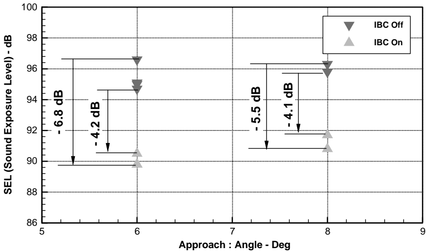
Figure 24. Reduction of sound exposure levels achieved by rotor active control for 6 and 8° approach flight procedures.
