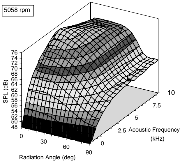
(a) Upstream radiation at 5058 rpm
