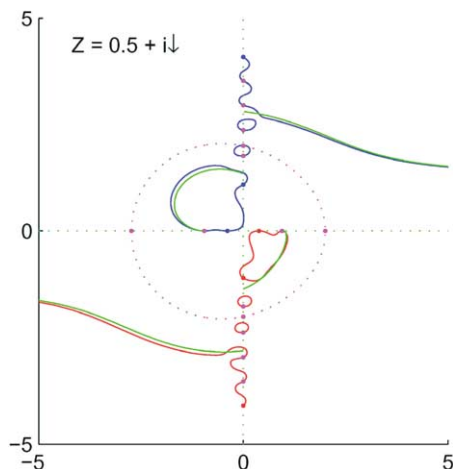
Figure 5. Trajectories of reduced wave number ( m = 1 , \omega = 5 ) for \text{Im}(Z) varying from \infty to -\infty and fixed \text{Re}(Z) = 0.5 . The 2-D surface wave limits are seen to be a very close approximation of the actual duct mode. The “egg” separates the regions of occurrence of the surface waves.
