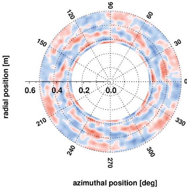
Figure 18. Instantaneous sound pressure pattern in the measurement plane for BPF_1 at 6 kHz, M = 0.3 .
