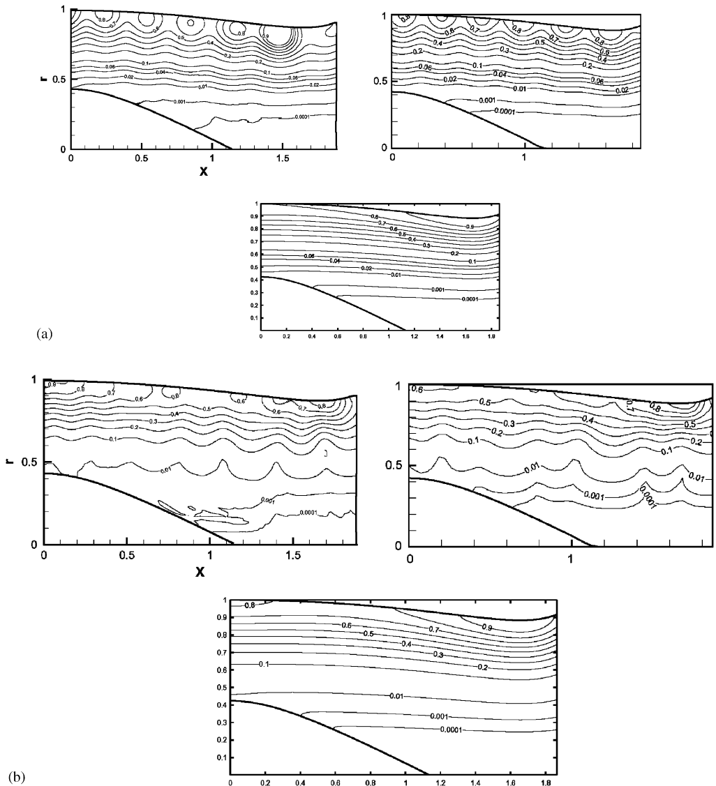
Figure 6. (a) Comparison of normalized pressure contours by CAA, FEM and MS, m = 10 , n = 1 , \sigma = 16 , and Ma = 0 . (b) Comparison of normalized pressure contours by CAA, FEM and MS, m = 10 , n = 1 , \sigma = 16 , and Ma = 0.5 .
