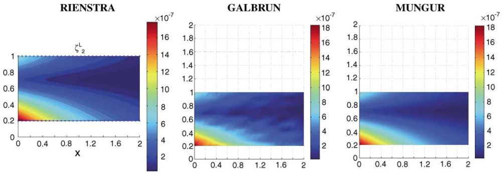
Figure 2. Comparisons results slowly varying duct: coupled FEM/BEM (Galbrun) and analytical benchmarks (Rienstra and Mungur).
