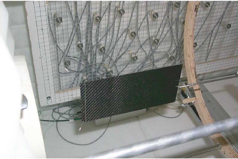
Figure 19. Experimental set-up for measurements of trailing-edge noise of a thin flat plate (AWD).
