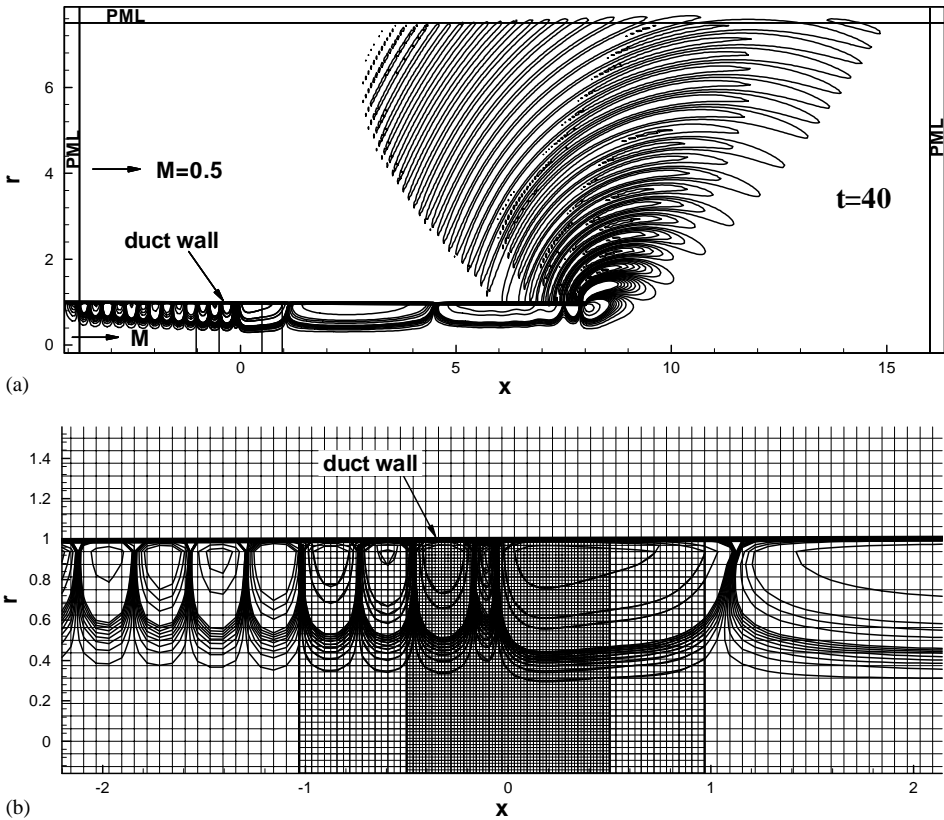
Figure 11. Pressure contour at t=40 and its enlarged plot close to grid interface; ducted rotor case with M=0.5 and \Omega=1.15 .
