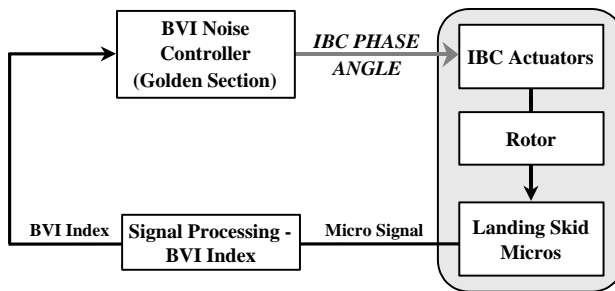
Figure 23. BVI noise control concept.
