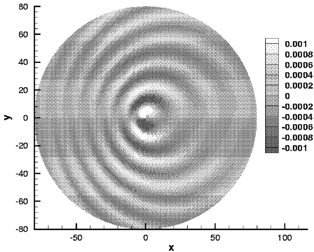
Figure 13. Unsteady pressure field using APEs with source term.
