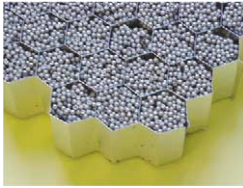
Example of new passive liner concept (Hollow sphere concept developed by METRAVIB).
