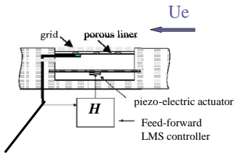
Example of adaptive liner concept (Acoustically adaptation developed by ECL and METRAVIB).
