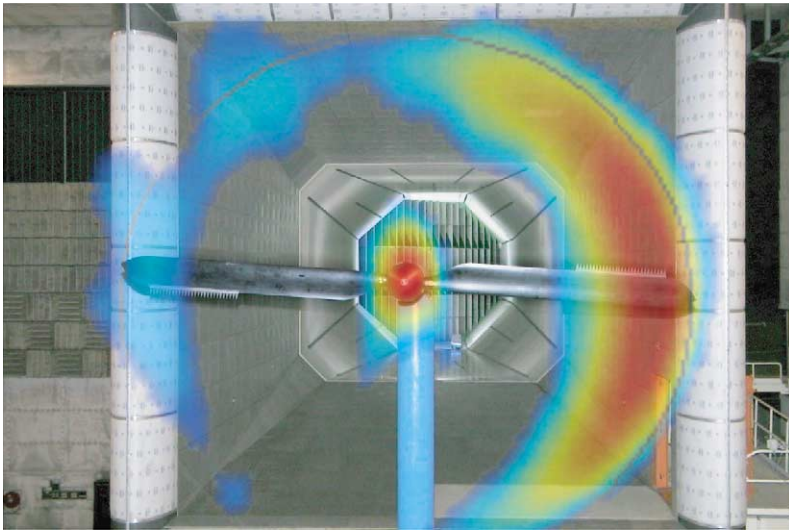
Figure 16. Acoustic image of model wind turbine at 8000 Hz, obtained with conventional array software.
