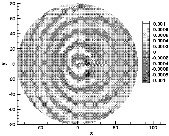
Figure 12. Unsteady perturbation pressure from high resolved CFD simulation.
