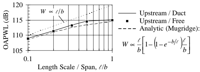
Figure 15. Effect of radial turbulence length scale on upstream radiation at 5058 r.p.m.: In-duct flow neglected, drag/thrust = 0.398.
