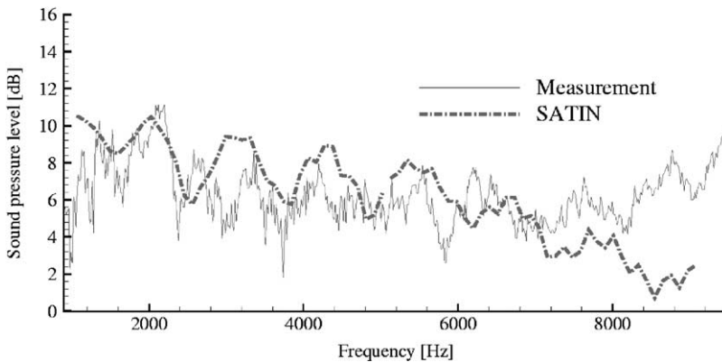
Figure 20. Measured and predicted sound spectra of a thin flat plate ( U_\infty = 36.3 m/s, c_f = 0.0037 , \delta = 4.8 mm).
