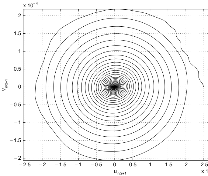
Figure 11. Whirling orbit versus time.
