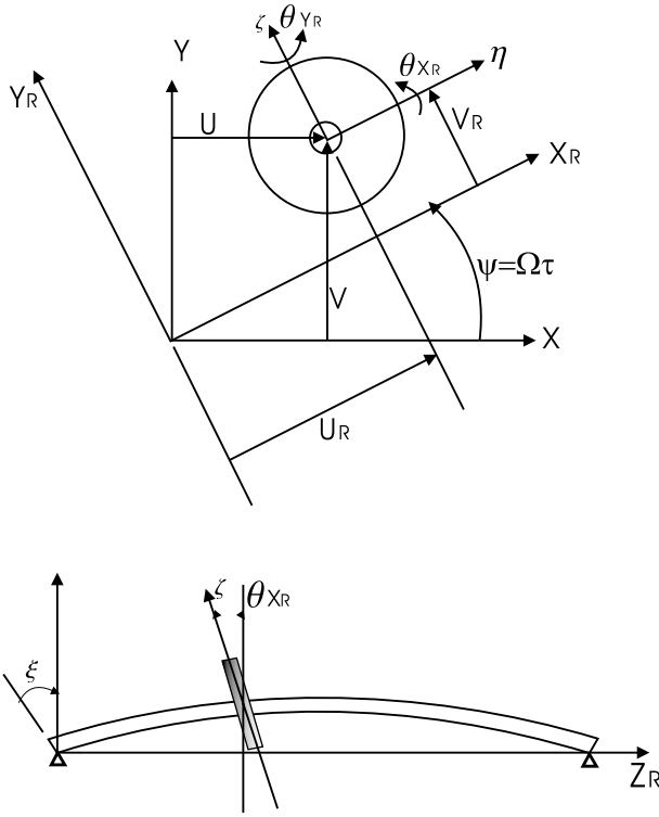
Figure 4. Schematic of a whirling rotor.
