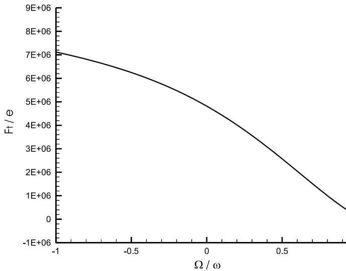
Figure 6. Aerodynamic force tangent to the offset versus whirling frequency.
