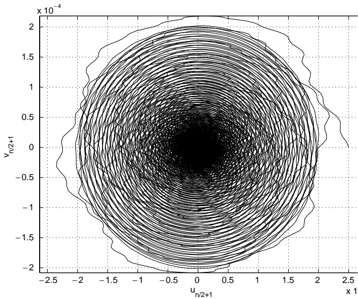
Figure 8. Whirling orbit versus time.
