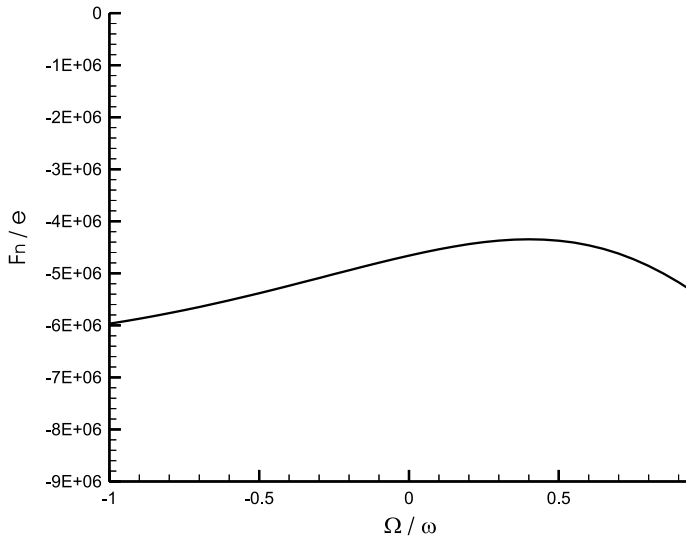
Figure 5. Aerodynamic force normal to the offset versus whirling frequency.
