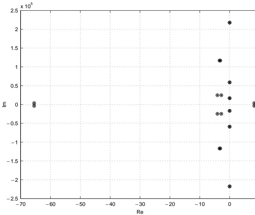
Figure 9. Root locus plot for the test rotor system without external loading.
