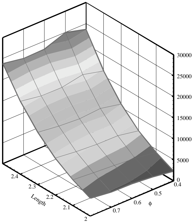
Figure 15. Stability boundary according to the flow coefficients and the shaft length.
