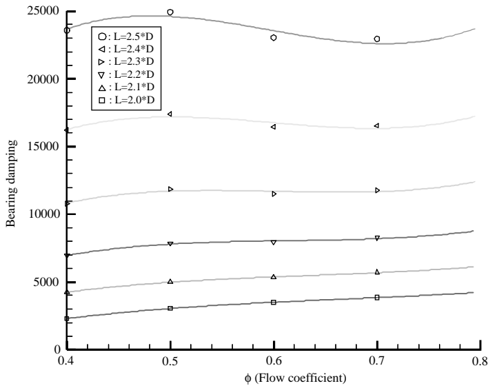
Figure 13. External damping required for neutral stability according to the flow coefficients.
