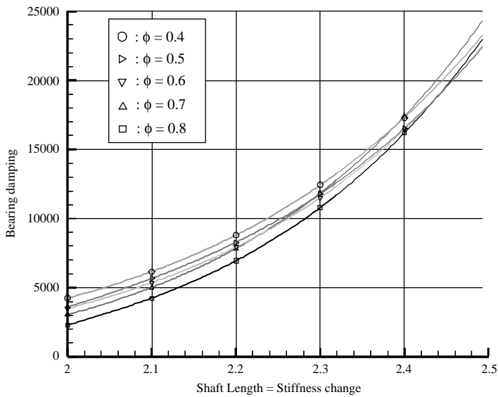
Figure 14. External damping required for neutral stability according to the shaft length.
