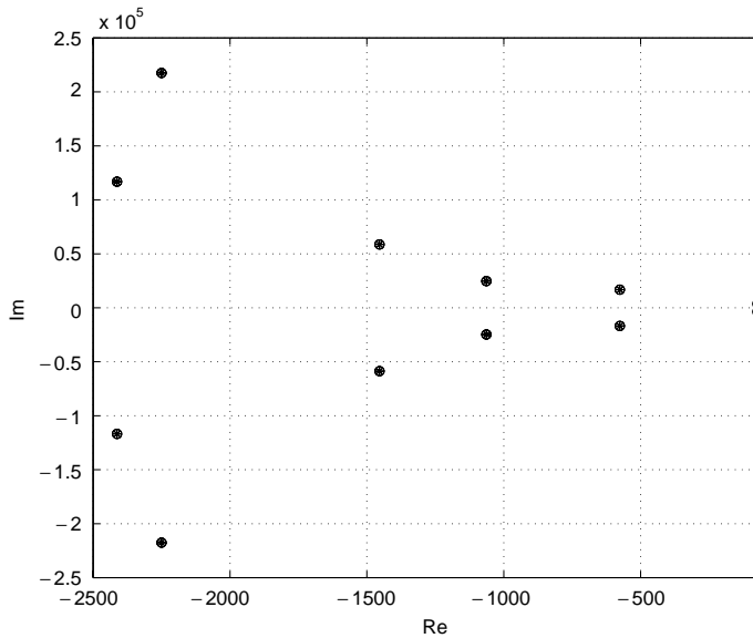
Figure 12. Root locus plot for the test rotor system with external damping of 3050 Ns/m.
