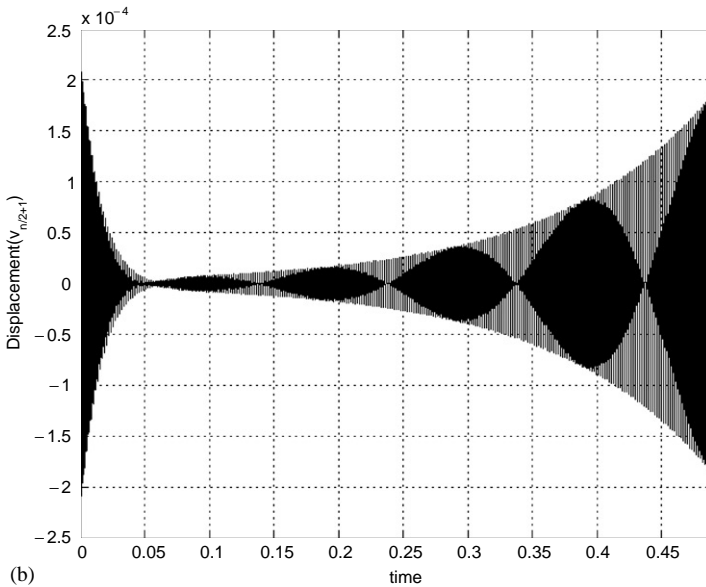
Figure 7. Displacement versus time without external damping ( L/D = 2.0 )
