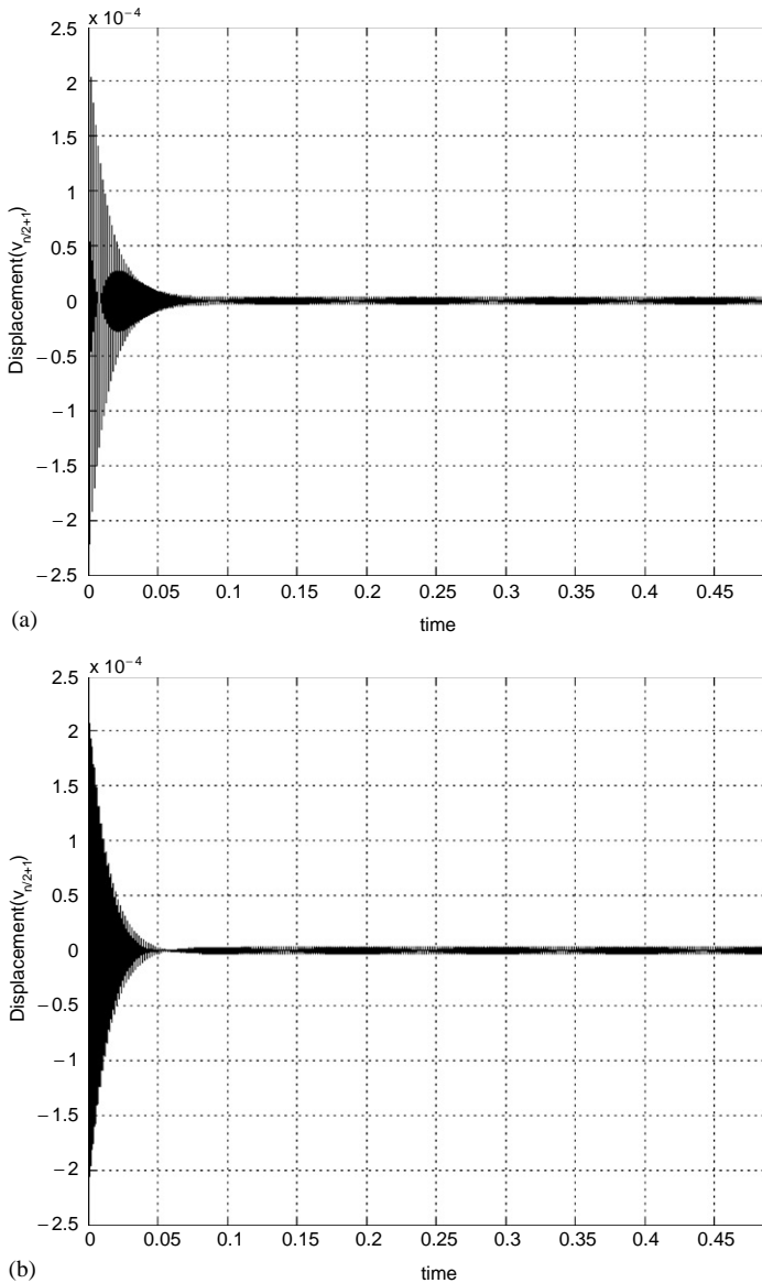
Figure 10. Displacement versus time with external damping of 3050 Ns/m ( L/D = 2.0 ).
