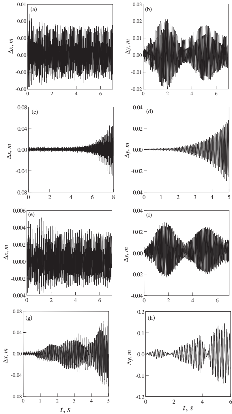
Fig. 2. Modes of vibration in time of the serpentine middle cross-section for different values of initial velocities of the entering fluid.
