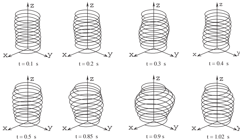
Fig. 3. Modes of the serpentine motions for case 8 in Table 1 ( V_0 = 27.2 m/s).
