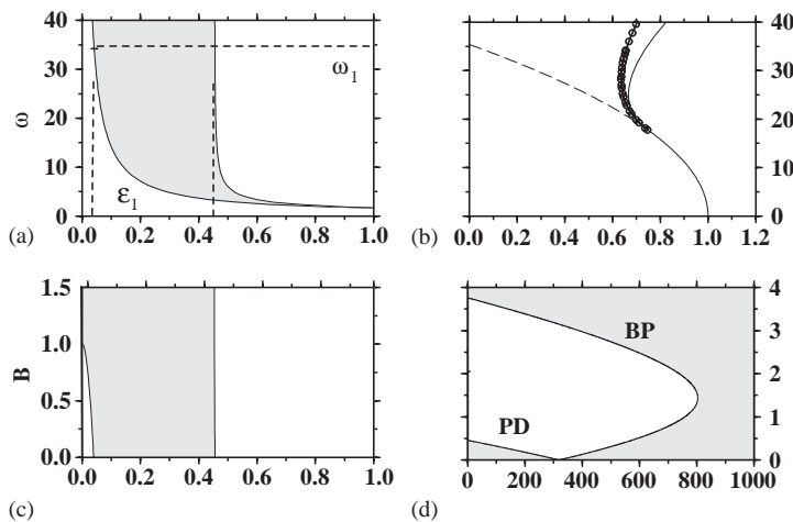
Fig. 3. Bifurcation diagrams for the single pendulum. Panel (a) is the \varepsilon - \omega bifurcation diagram for B = 0 and \Gamma = 0.1 . Panel (b) is the position of the pitchfork bifurcation in the \omega - B plane for a fixed value of \varepsilon . We have chosen \varepsilon = 0.04 and marked it in panel (a) with the symbol \varepsilon_1 and the corresponding frequency with \omega_1 . See text for explanation of the curves emanating from the codimension-two point. Panel (c) shows the \varepsilon - B bifurcation diagram for a fixed value of the frequency, marked by \omega_1 in panel (a). The shaded region corresponds to stability of the inverted pendulum position. Panel (d) plots the (\varepsilon, B) -bifurcation diagram corresponding to the same values as those used in (c) but in a broader range.
