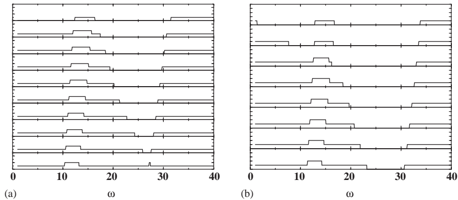
Fig. 7. Number of characteristic multipliers outside the unit circle for N = 8 (a) and N = 16 (b), \Gamma = 0.004 and decreasing values of B . The upper curves correspond to the critical value and the system of pendulums are stable even for vanishing frequencies. As the elastic component is lowered, the stability regions shrink. The small plateaus with 2 characteristic multipliers outside the unit circle reveal further bifurcations of the already unstable system.
