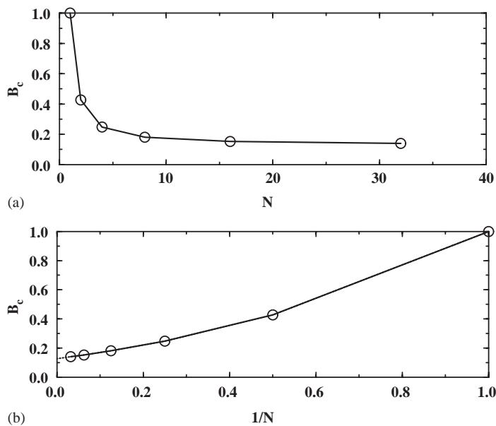
Fig. 4. The upper part of the figure shows the critical values of B as a function of the number of pendulums N . They approach the value corresponding to the continuum limit ( B_{\infty} = 0.1278 ) in an asymptotic way. The lower figure shows the same quantity as a function of 1/N to make the scaling behaviour more evident. The dashed line is the quadratic extrapolation to the origin that gives an estimation of B = 0.1275 for the critical value of the elastic coefficient.
