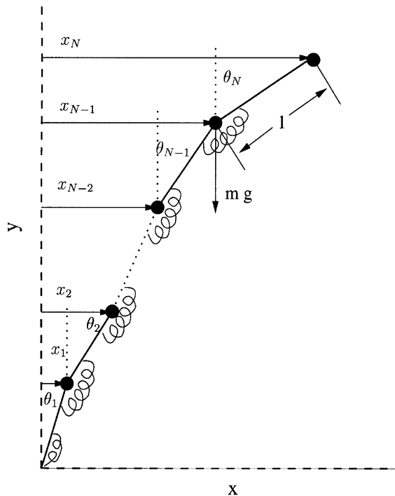
Fig. 1. Model of N identical pendulums. Each pendulum has length l and mass m and there is an elastic spring at each joint. The variable \theta_i measures the angle with respect to the previous shaft whereas the generalized co-ordinate x_i measures the horizontal distance to the vertical position of the bob i .
