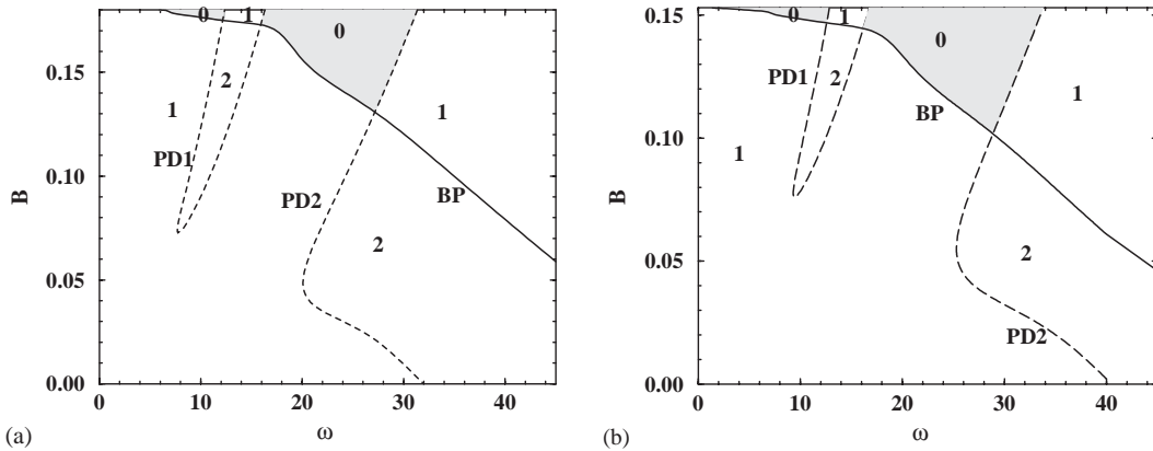
Fig. 8. B - \omega bifurcation set for fixed \varepsilon = 0.02 , \Gamma = 0.004 , N = 8 (left) and N = 16 (right). The digits inside each region denote the number of multipliers outside the unit circle. The stable regions have been shaded and are limited by curves of pitchfork (BP) and period doubling bifurcations (PD). A schematic representation of the mode that becomes unstable is also included at several points in the diagram.
