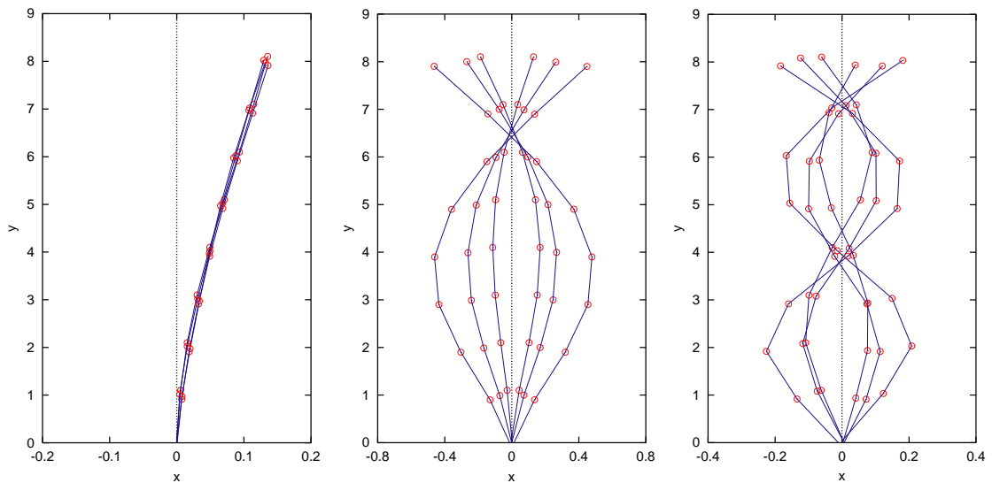
Fig. 9. Representation of the modes that become unstable for N = 8 pendulums when crossing the borders in the B - \omega bifurcation diagram at the curves labeled by BP, PD1 and PD2, respectively. Snapshots of the multiple pendulums are shown at different instants of time within a period.
