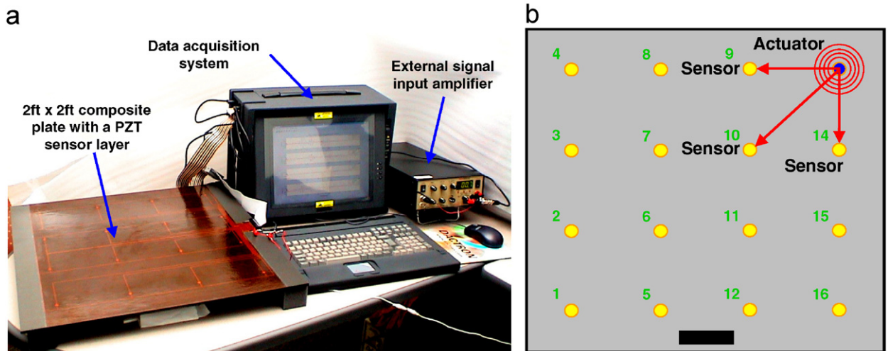
Fig. 9. An active sensing system for detecting delamination on a composite plate: (a) testing configuration and (b) the layout of the PZT sensors/actuators.
