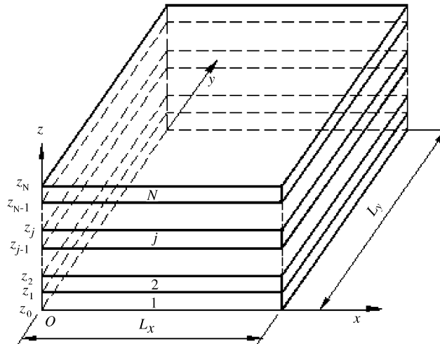
Fig. 1. The magneto-electro-elastic layered plate.
