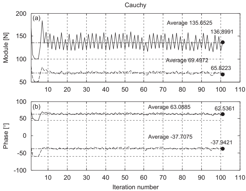
Fig. 14. Estimated values vs. iteration for the Cauchy's estimate: (a) force amplitudes and (b) force phases.
