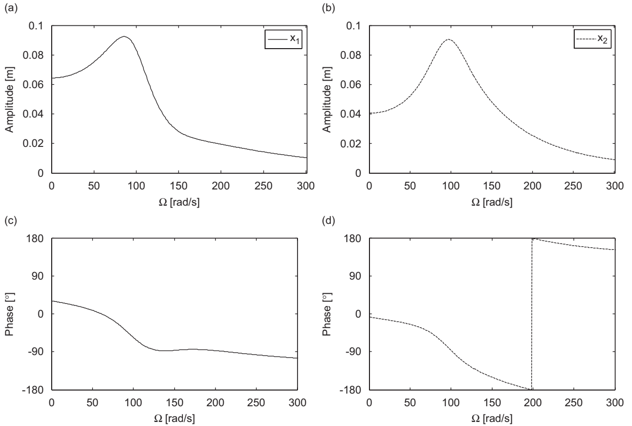
Fig. 6. Nominal response of the system: (a) amplitude of x_1 , (b) amplitude of x_2 , (c) phase of x_1 and (d) phase of x_2 .
