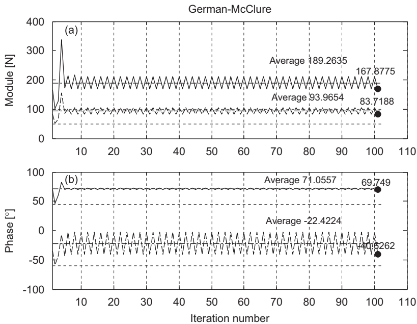
Fig. 15. Estimated values vs. iteration for the German-McClure's estimate: (a) force amplitudes and (b) force phases.
