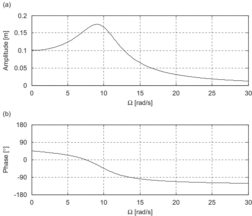
Fig. 2. Nominal response of the system: (a) amplitude and (b) phase.
