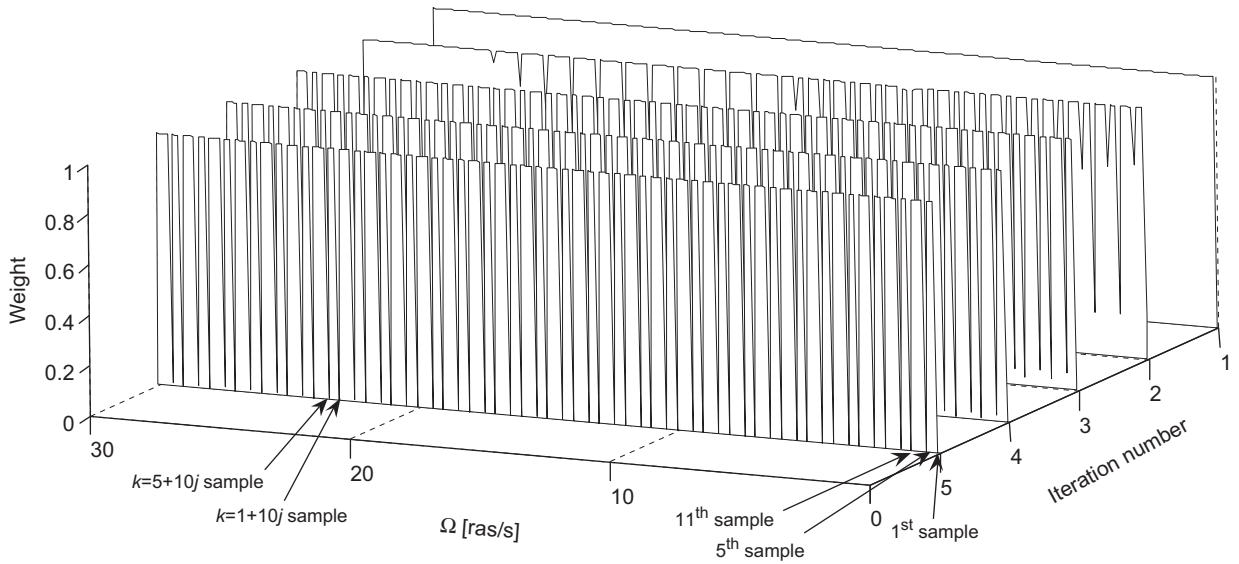
Fig. 4. Weights attributed per iteration for the Huber's estimator.
