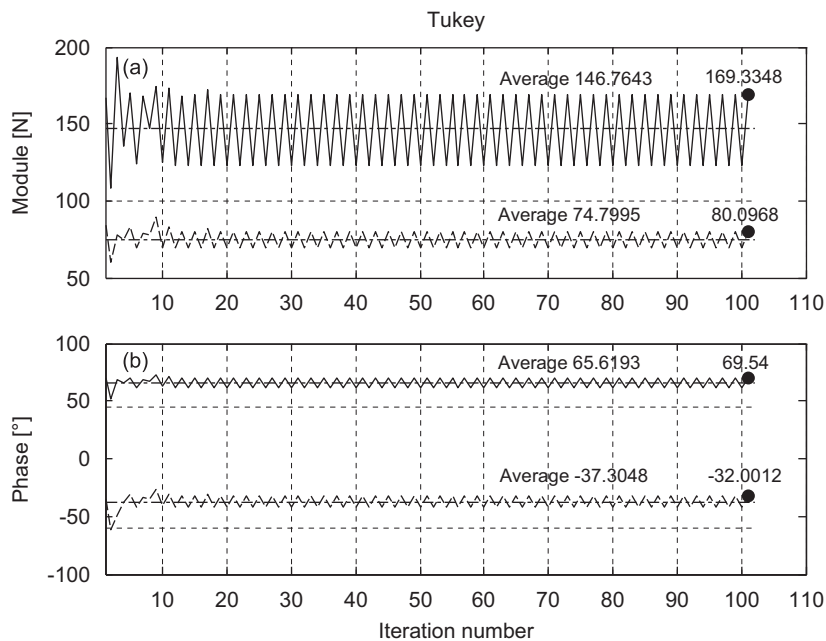
Fig. 17. Estimated values vs. iteration for the Tukey's estimate: (a) force amplitudes and (b) force phases.
