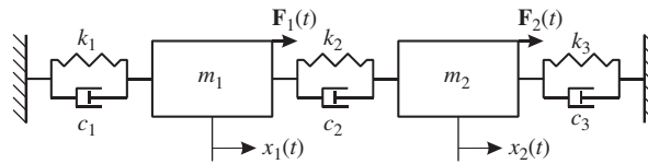
Fig. 5. System with 2 degrees of freedom.
