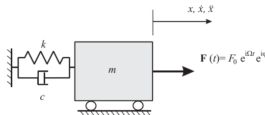
Fig. 1. Single degree-of-freedom system.
