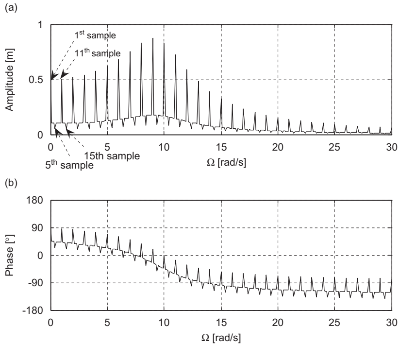
Fig. 3. Corrupted response of the system: (a) amplitude and (b) phase.
