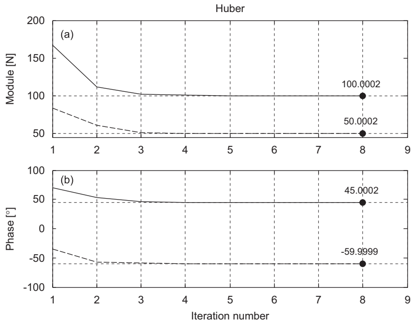
Fig. 12. Estimated values vs. iteration for the Huber's estimate: (a) force amplitudes and (b) force phases.
