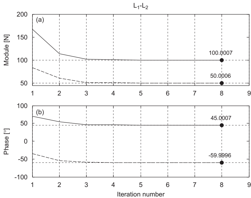
Fig. 9. Estimated values vs. iteration for the L_1-L_2 estimate: (a) force amplitudes and (b) force phases.
