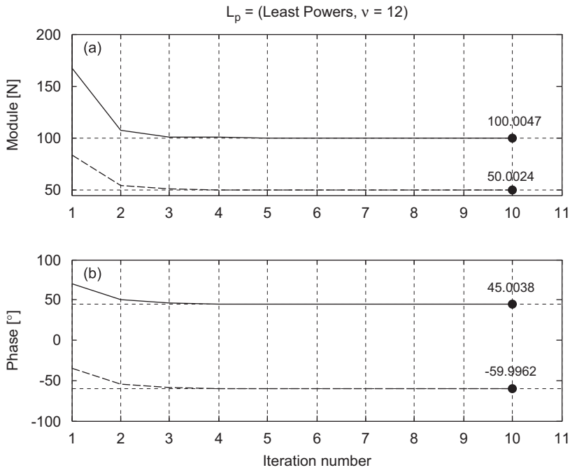
Fig. 10. Estimated values vs. iteration for the L_p estimate: (a) force amplitudes and (b) force phases.
