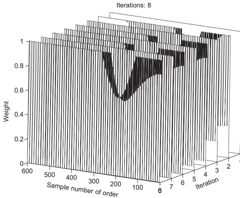
Fig. 18. Weights attributed per iteration for the Huber's estimate.
