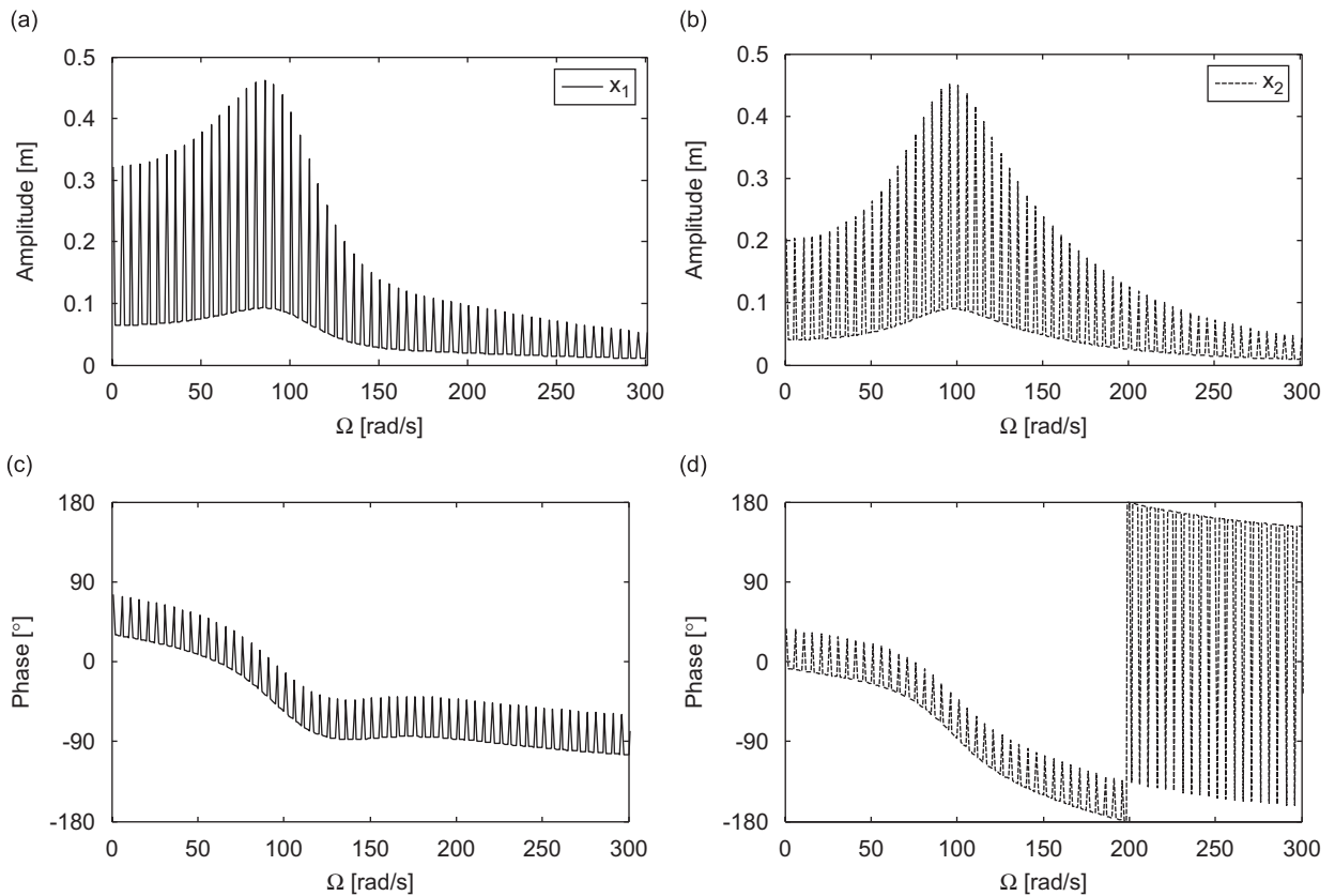
Fig. 7. Corrupted response of the system: (a) amplitude of x_1 , (b) amplitude of x_2 , (c) phase of x_1 and (d) phase of x_2 .
