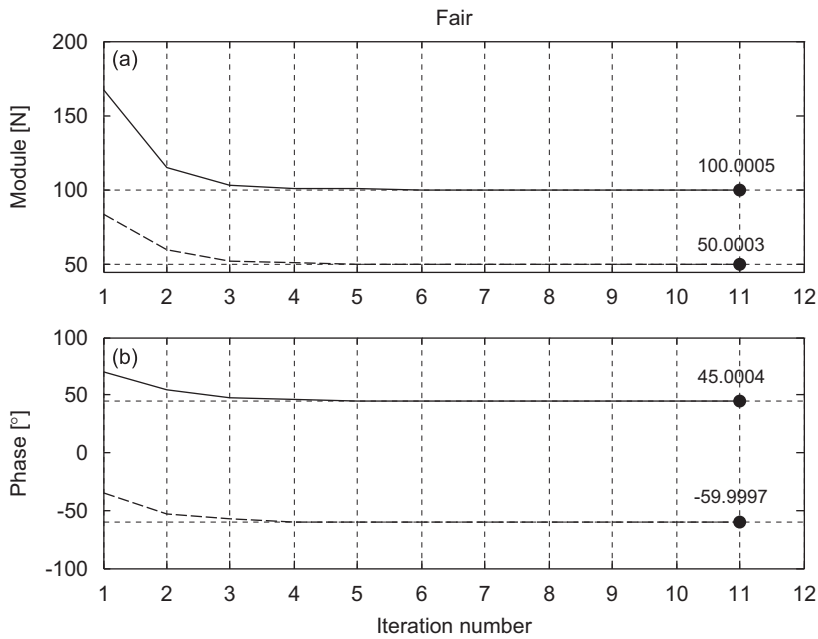
Fig. 11. Estimated values vs. iteration for the Fair estimate: (a) force amplitudes and (b) force phases.
