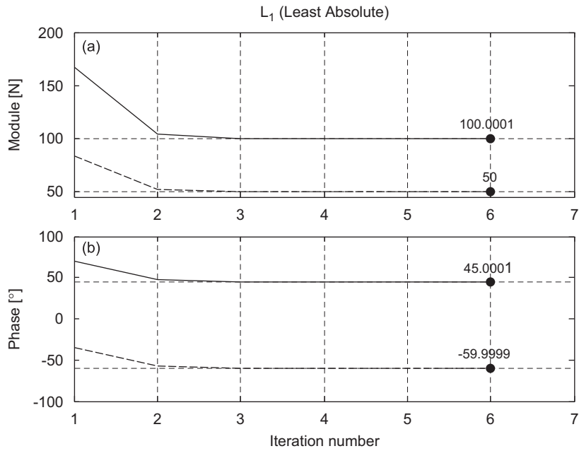
Fig. 8. Estimated values vs. iteration for the L_1 estimate: (a) force amplitudes and (b) force phases.
