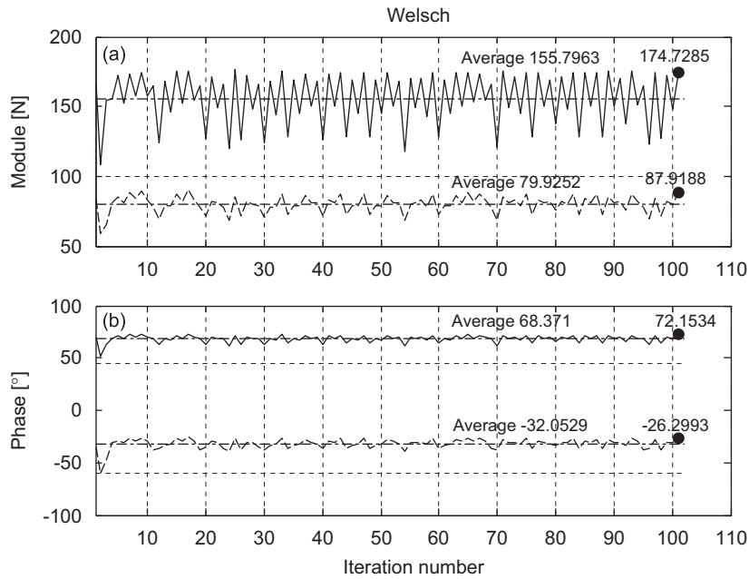
Fig. 16. Estimated values vs. iteration for the Welsch's estimate: (a) force amplitudes and (b) force phases.
