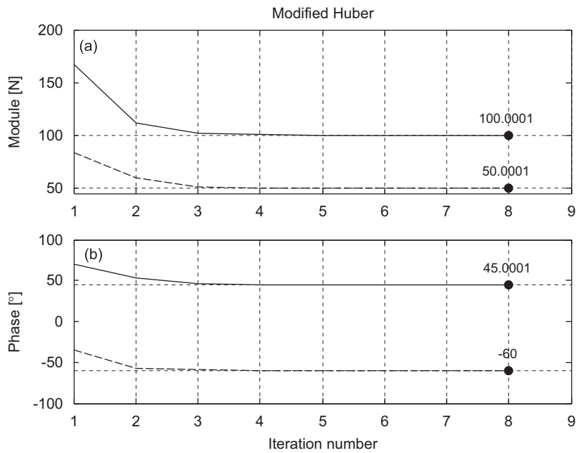
Fig. 13. Estimated values vs. iteration for the Modified Huber's M-estimate: (a) force amplitudes and (b) force phases.
