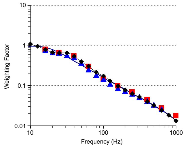
Fig. 5. Comparisons of the ISO-frequency weighting [1] and the vibration power absorption-based frequency weightings ((—●—) ISO weighting [1]; (—◆—) vibration power absorption weighting derived from the impedance data in Ref. [29]; (—▲—) vibration power absorption weighting derived from the impedance data in Ref. [25]; and (—■—) vibration power absorption weighting reported in Ref. [10]).
