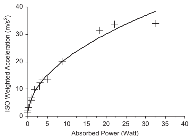
Fig. 4. Correlation relationship between the ISO-weighted accelerations and the total vibration power absorption values predicted with Eq. (1) for the 20 sets of tool vibration data reported in Ref. [26] ((+ + + + +) raw data; (—) trendline).
