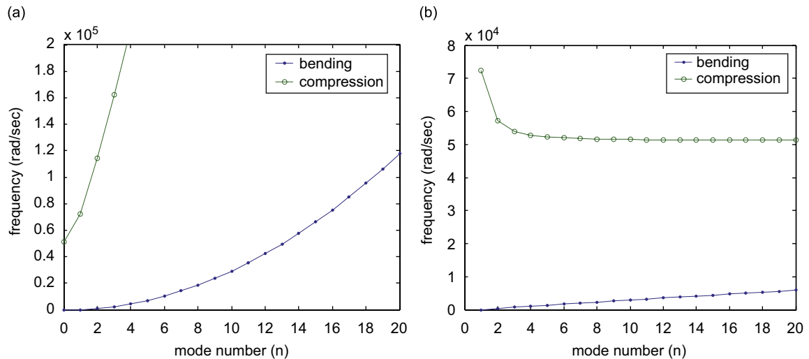
Fig. 2. Natural frequencies vs. mode number for (a) stationary normal mode shapes and (b) quasi-stationary mode shapes.
