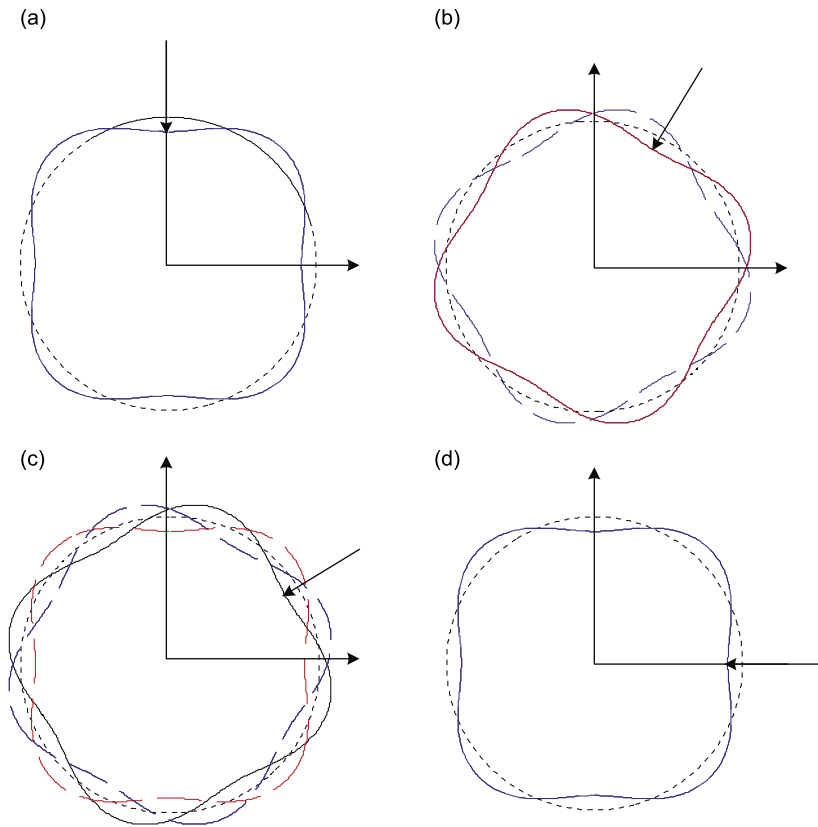
Fig. 3. Wave forms set up by travelling point load, forward travelling waves —, and backward travelling waves ----.
