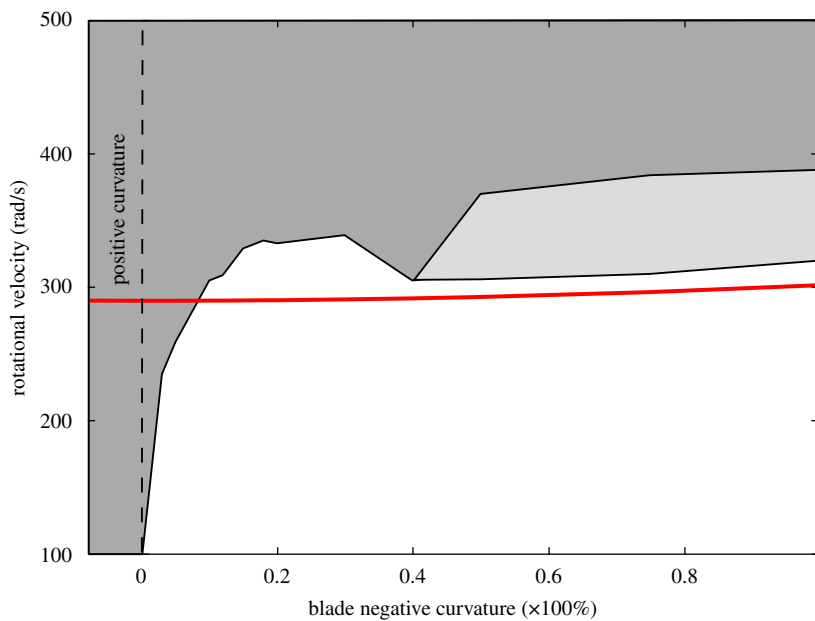
Fig. 21. The different possible vibratory behaviors of the structures are given with respect to the blades curvature and the rotational velocity; N = 22 , k = 3 and \mu = 1 ; (□) damped, (□) sustained, (■) divergent, and (—) analytical solution.
