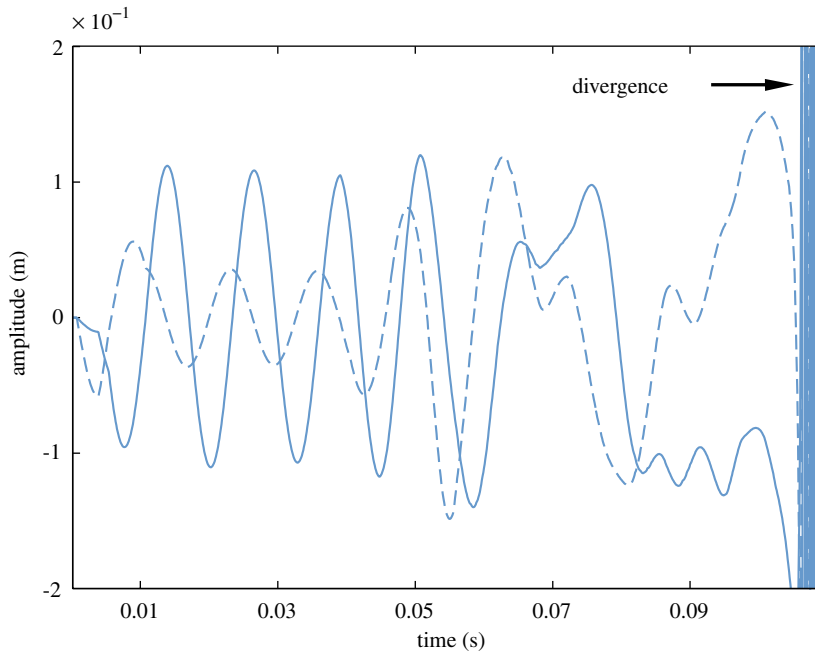
Fig. 14. vibrations of the two modes of the bladed disk for \Omega = 351.8 \text{ rad/s} ( \Omega > \Omega_{cn} ): u_{m,b}^1 (----) and u_{m,b}^2 (—). The amplitudes of vibration diverge very quickly.
