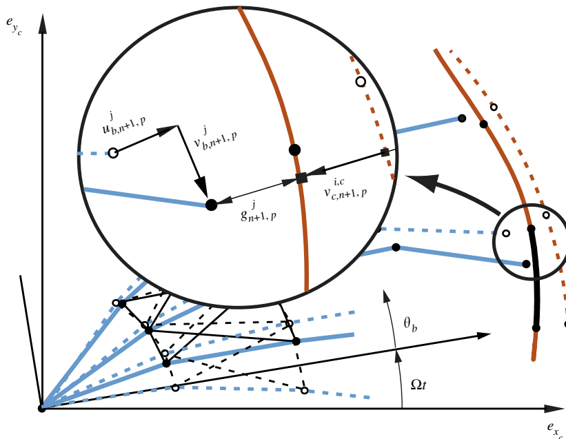
Fig. 7. Initial (---) and current predicted (—) configurations of a part of the bladed disk and casing.
