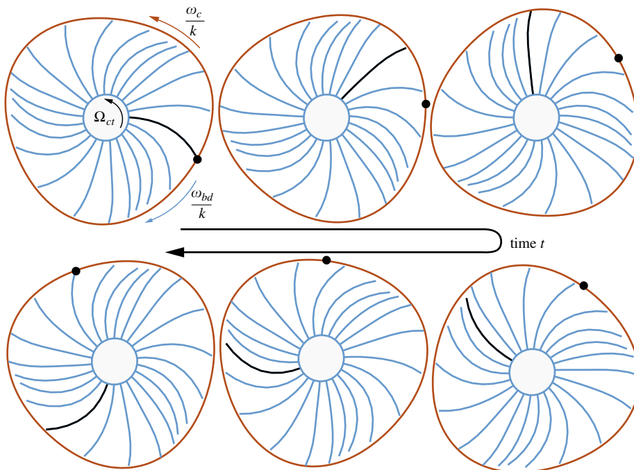
Fig. 4. Schematic of a modal interaction coincidence for k = 3 . The bladed disk rotates clockwise at \Omega_{ct} as shows the black blade. From a stationary frame, a forward rotating 3-nodal diameter mode propagates at \omega_c/k in the casing (marked by a black dot) and its counter-rotating counterpart at \Omega_{ct} - \omega_{bd}/k in the bladed disk.
