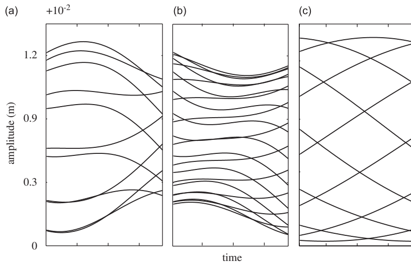
Fig. 8. Distances between the casing and the N = 22 blade-tips before contact is initiated. The time scale is not of interest. A forward k -nodal diameter mode is rotating on the casing and a counter-rotating one on the bladed disk. (a) k = 2 , 11 curves are distinguishable; (b) k = 3 , 22 curves are distinguishable; (c) k = 4 , 11 curves are distinguishable. The number of distinguishable curves shows the symmetry of the system in terms of future contact locations between the two components versus N and k .
