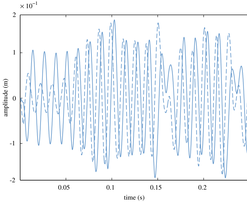
Fig. 12. Vibrations of the two modes of the bladed disk for \Omega = 351.4 \text{ rad/s} ( \Omega \simeq \Omega_{cn} ): u_{m,b}^1 (----) and u_{m,b}^2 (—). A counter-rotating mode propagates in the bladed disk.
