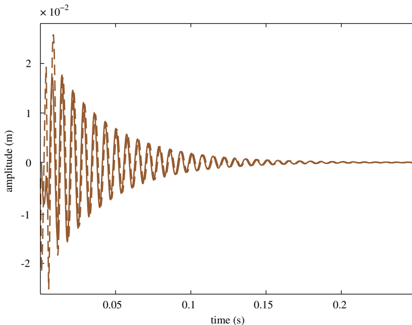
Fig. 9. Vibrations of the two modes of the casing for \Omega = 350.2 rad/s ( \Omega < \Omega_{cn} ): u_{m,c}^1 (---) and u_{m,c}^2 (—). A decaying behavior of the casing is observed due to the presence of structural damping in the model.
