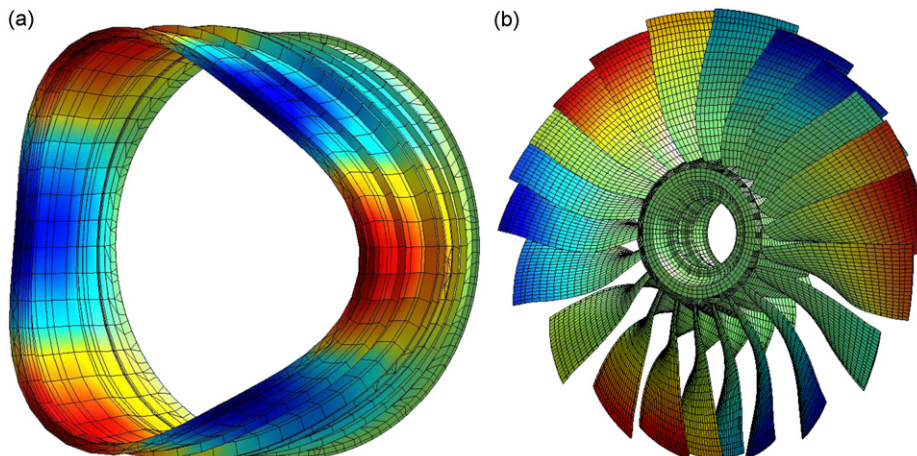
Fig. 2. 3-nodal diameter modes of (a) a jet engine casing and (b) a bladed disk.
