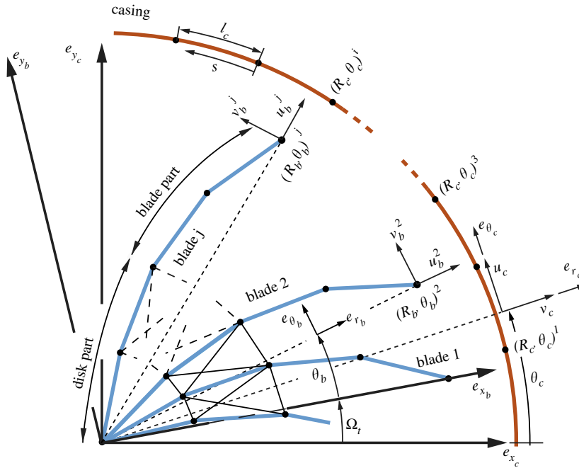
Fig. 5. Schematic of the reference configuration of the bladed disk and casing in their respective frame (e_{x_b}, e_{y_b}) and (e_{x_c}, e_{y_c}) .
