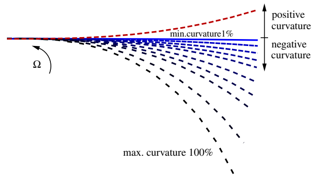
Fig. 20. Classification of the tested blade curvatures from 1% (almost straight) to 100% (highly curved). A blade with positive curvature is also plotted.
