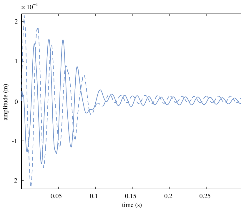
Fig. 18. Vibrations of the two modes of the bladed disk for \Omega = 110 rad/s ( \Omega > \Omega_c ): u_{m,b}^1 (---) and u_{m,b}^2 (—). They are decaying until a static deformed state is reached.
