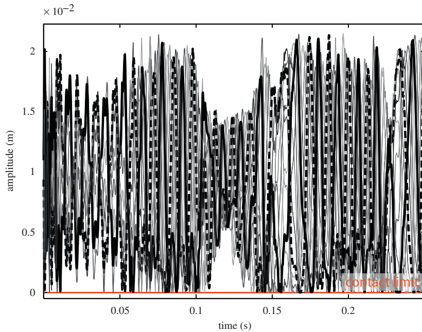
Fig. 16. Distances between the casing and blade-tips for N = 22 , k = 3 and \Omega = 351.4 rad/s. The intermittent behavior can be observed for two highlighted blades (dash and solid bold black lines).
