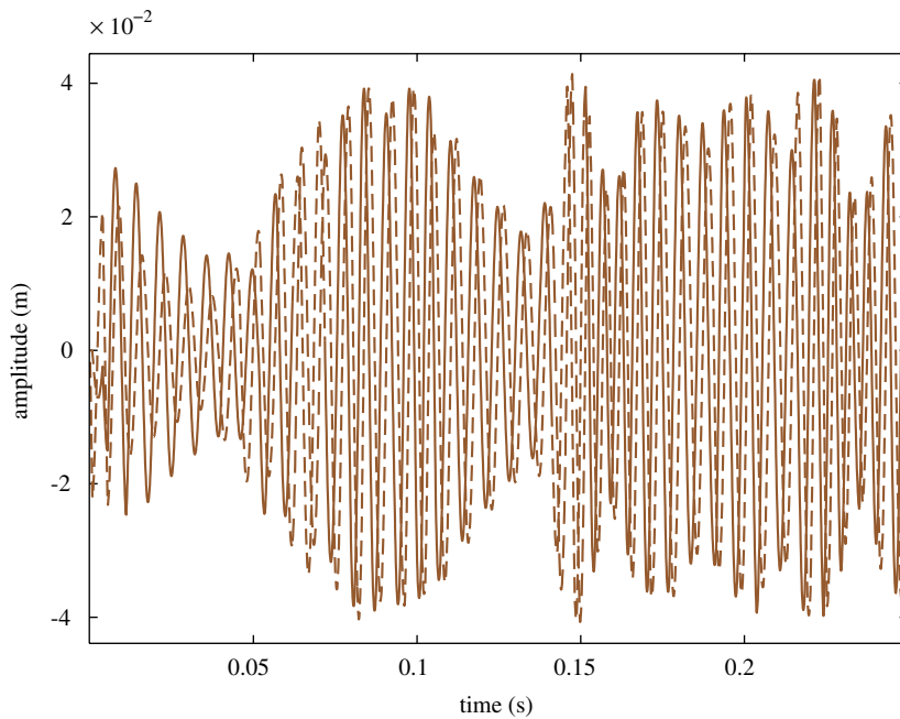
Fig. 11. Vibrations of the two modes of the casing for \Omega = 351.4 \text{ rad/s} ( \Omega \simeq \Omega_{cn} ): u_{m,c}^1 (---) and u_{m,c}^2 (—). A forward rotating mode propagates in the casing.
