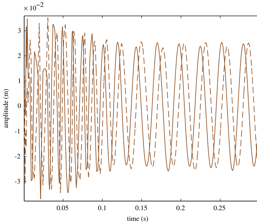
Fig. 17. Vibrations of the two modes of the casing for \Omega = 110 rad/s ( \Omega > \Omega_{cn} ): u_{m,c}^1 (---) and u_{m,c}^2 (—). A forward rotating mode starts traveling after 0.14 s of simulation.
