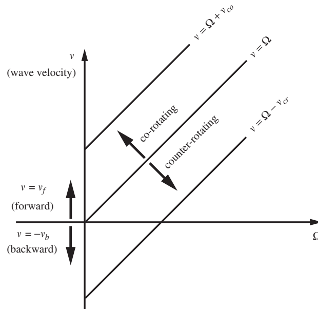
Fig. A.1. Wave velocity versus rotational velocity diagram explaining directional terms.
