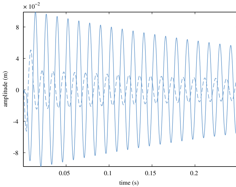
Fig. 10. Vibrations of the two modes of the bladed disk for \Omega = 350.2 \text{ rad/s} ( \Omega < \Omega_{cn} ): u_{m,b}^1 (---) and u_{m,b}^2 (—). A decaying behavior of the bladed disk is observed due to the presence of structural damping in the model.
