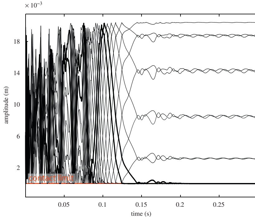
Fig. 19. Distances between the casing and the blade tips for \Omega = 110 \text{ rad/s} . Due to the symmetry of the system, only 11 curves are distinguishable. After 0.14 s of simulation, four blades (4 solid bold black curves are shown but only 2 are distinguishable) come in permanent contact against the casing and push a forward rotating mode.
