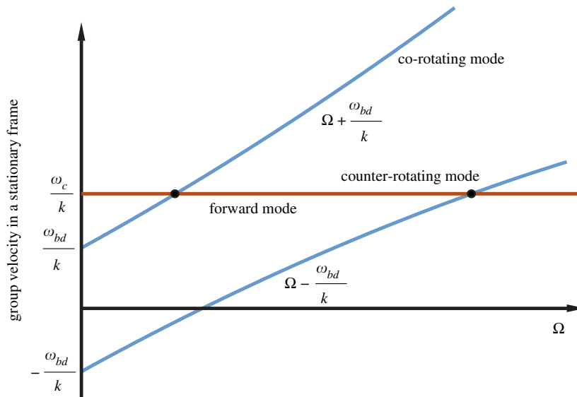
Fig. 3. Theoretical modal interaction conditions • as an extension of a Campbell diagram for k -nodal diameter modes. The frequency \omega_c is usually greater than \omega_{bd} of the first flexural mode of the blades. Both lines of equation \Omega \pm \omega_{bd}/k are normally curved as \omega_{bd} is \Omega -dependent: in our study, they are considered as straight lines, meaning that no centrifugal stiffening is accounted for.
