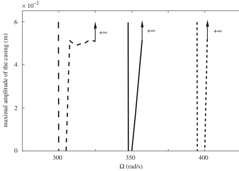
Fig. 15. Critical rotational velocities, with on the left, the analytical value and on the right, the numerical value; (—): k = 3 , \Omega_{ct} = 301.56 ; (—): k = 4 , \Omega_{ct} = 343.58 ; (- - -): k = 5 , \Omega_{ct} = 390.37 .
