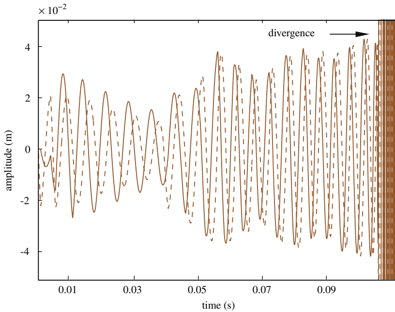
Fig. 13. Vibrations of the two modes of the casing for \Omega = 351.8 \text{ rad/s} ( \Omega > \Omega_{cn} ): u_{m,c}^1 (----) and u_{m,c}^2 (—). The amplitudes of vibration diverge very quickly.
