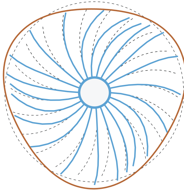
Fig. 6. 3-nodal diameter modes of the casing and the bladed disk.
